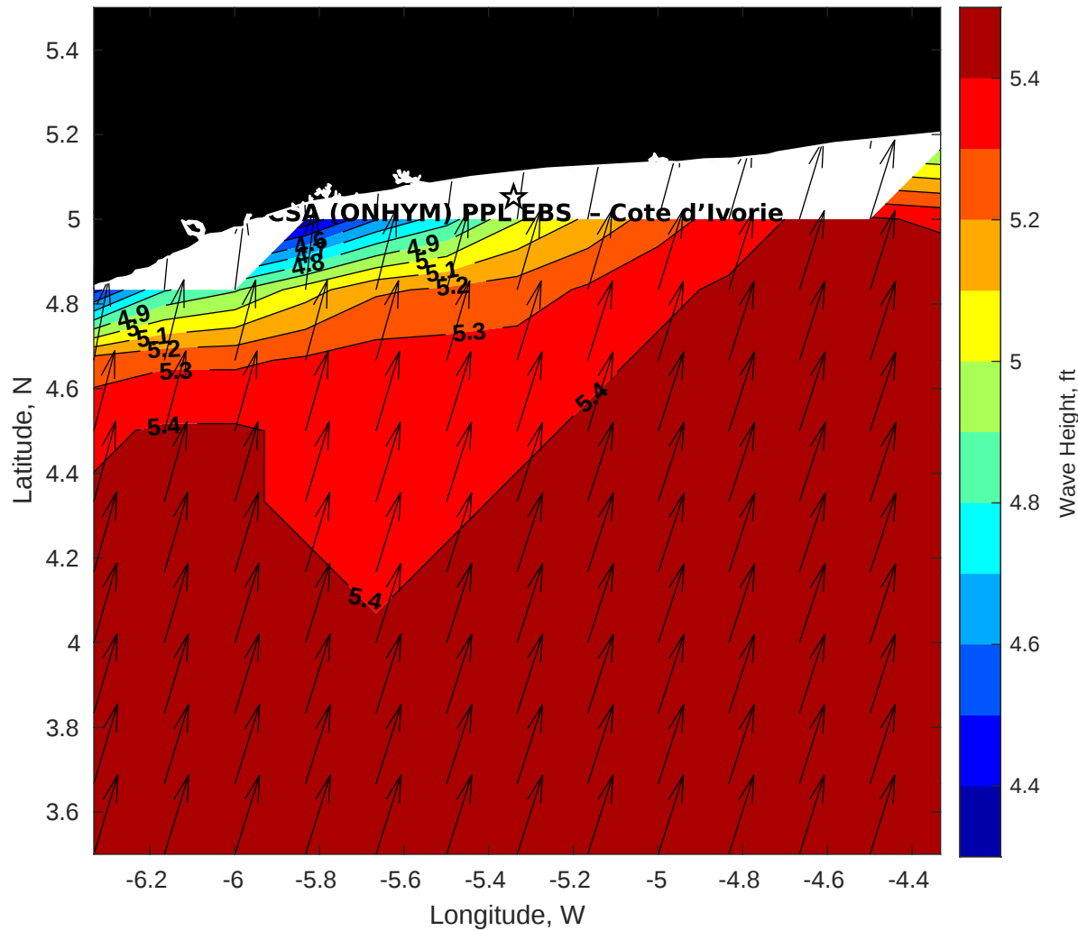
Wave Height (ft) for CSA (ONHYM) PPL EBS - Cote d'Ivoire at 14-Jul-2025 09:00:00
