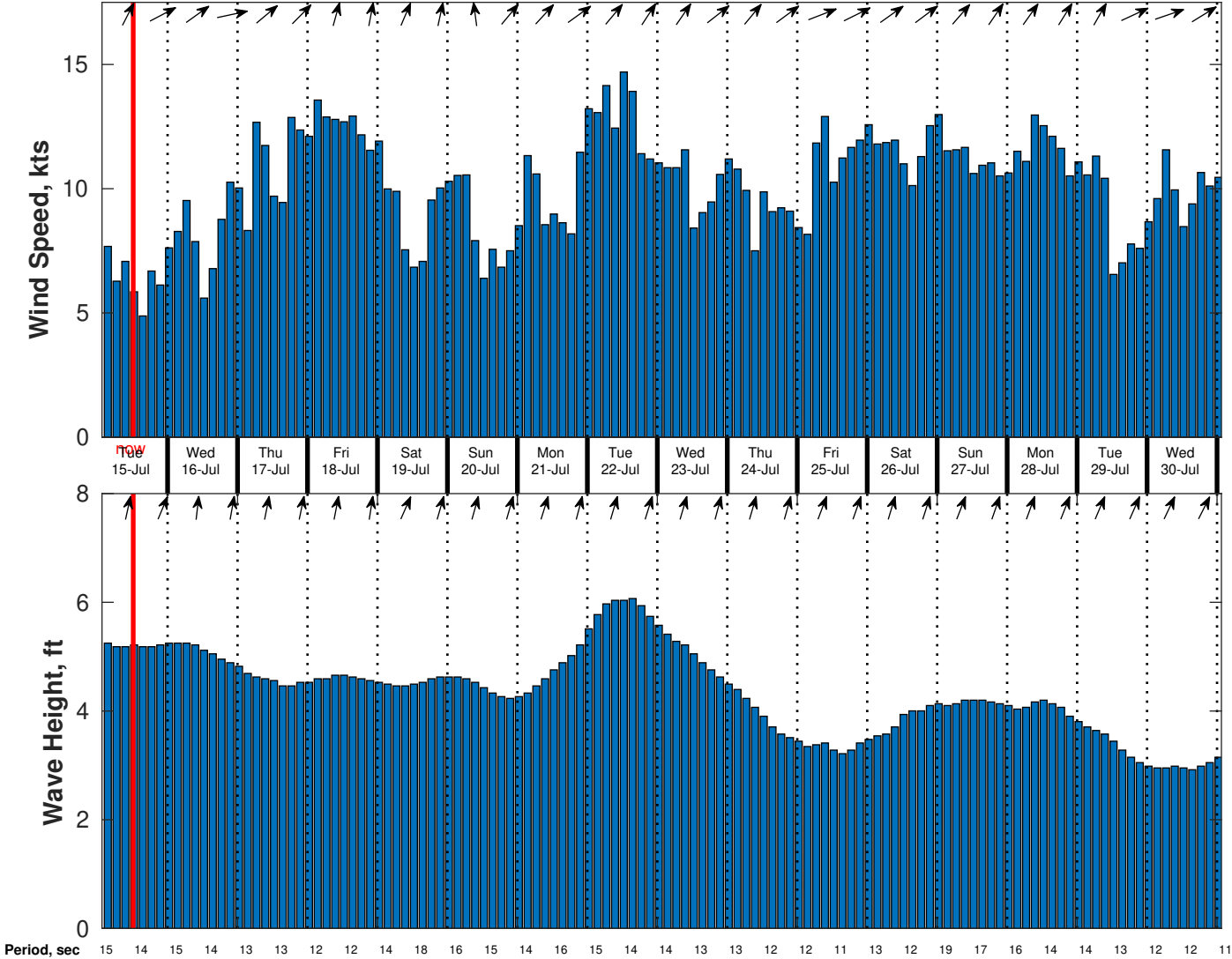
Wind & Wave Forecast for CSA (ONHYM) PPL EBS - Ghana from 14-Jul-2025 02:00:00 to 30-Jul-2025 02:00:00
