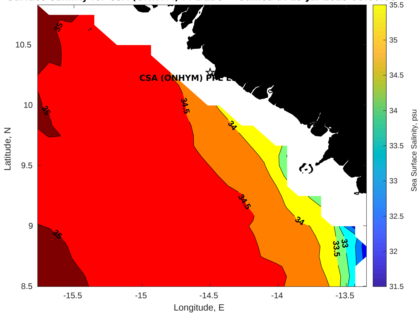
Surface Salinity for CSA (ONHYM) PPL EBS - Guinea at 13-Jul-2025 00:00:00
