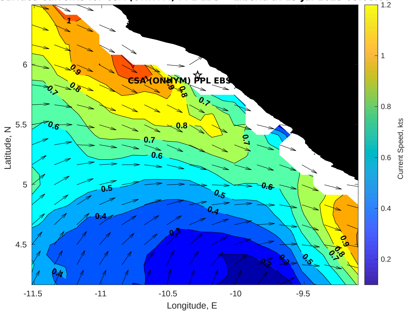
Surface Currents for CSA (ONHYM) PPL EBS - Liberia at 13-Jul-2025 00:00:00
