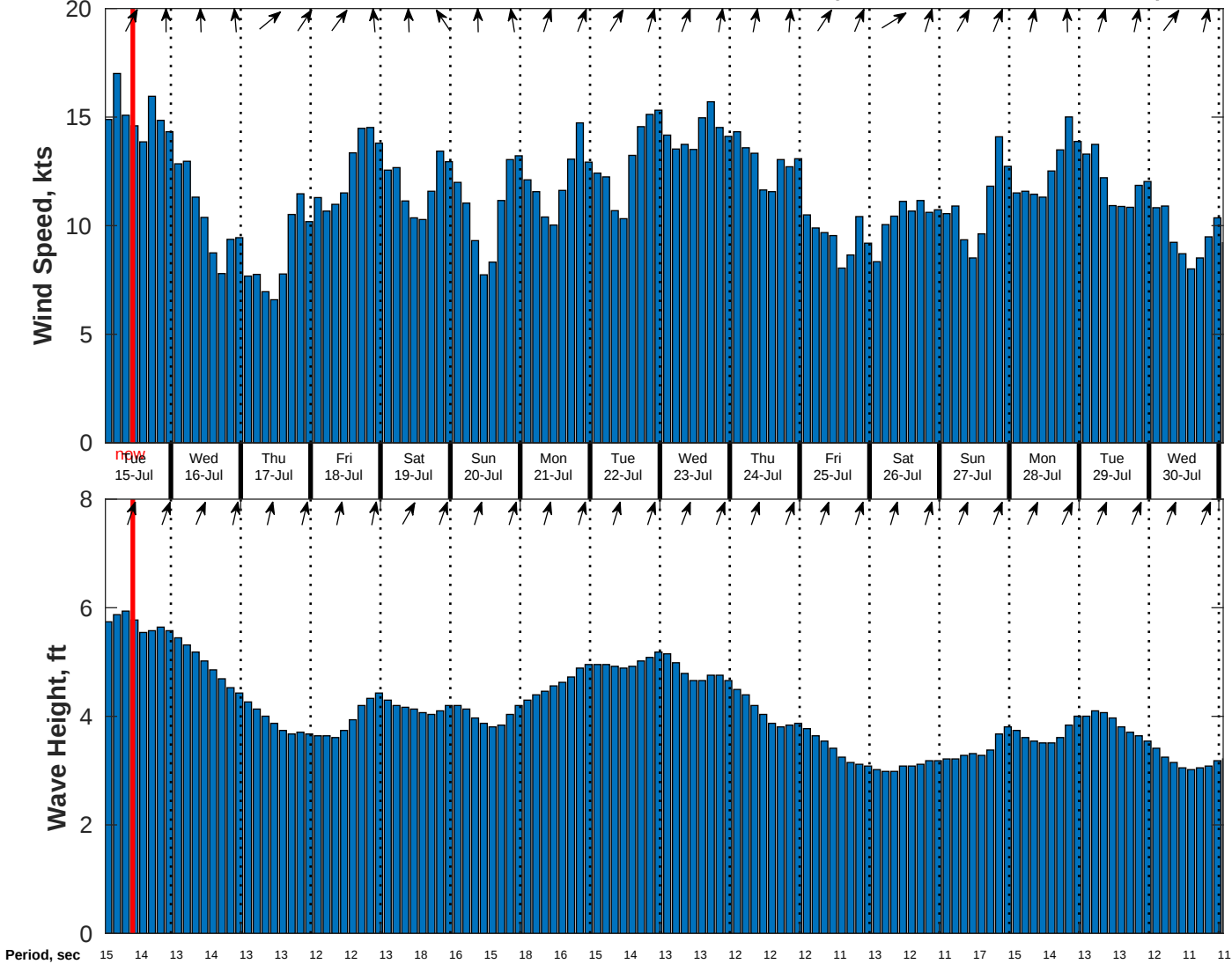
Wind & Wave Forecast for CSA (ONHYM) PPL EBS - Liberia from 14-Jul-2025 01:00:00 to 30-Jul-2025 01:00:00
