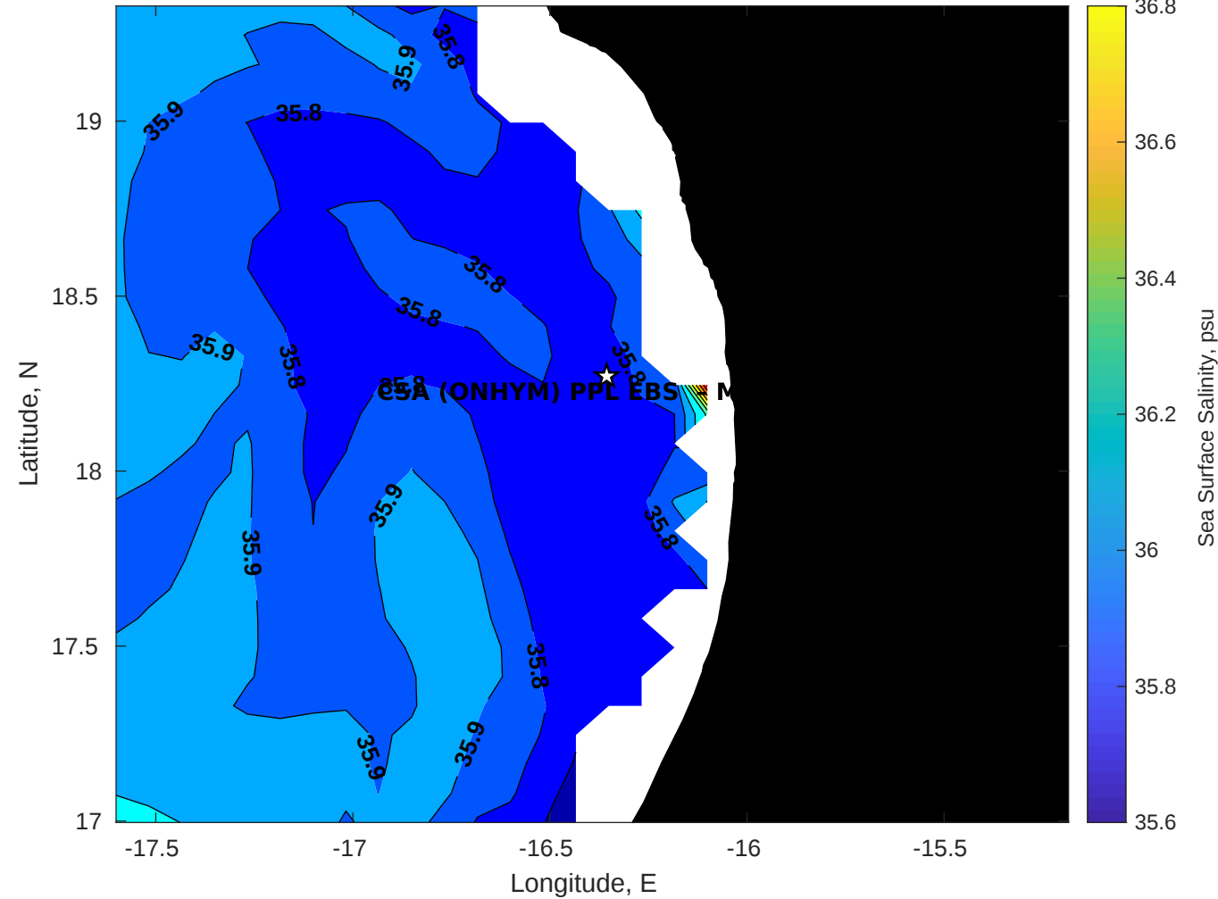
Surface Salinity for CSA (ONHYM) PPL EBS - Mauritania at 13-Jul-2025 00:00:00
