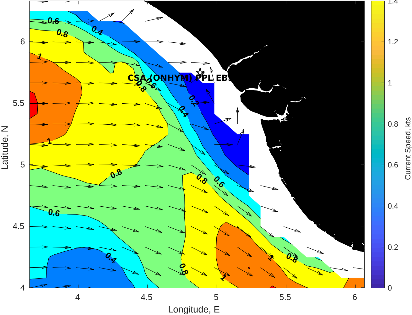
Surface Currents for CSA (ONHYM) PPL EBS - Nigeria at 13-Jul-2025 00:00:00
