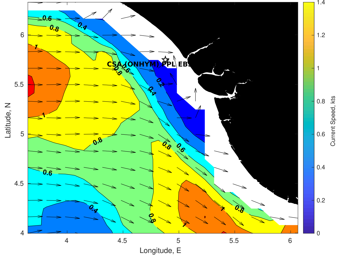
Surface Currents for CSA (ONHYM) PPL EBS - Nigeria at 13-Jul-2025 00:00:00
