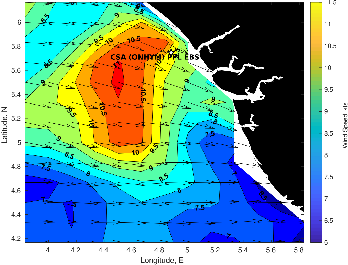
Winds (kts) for CSA (ONHYM) PPL EBS - Nigeria at 14-Jul-2025 09:00:00
