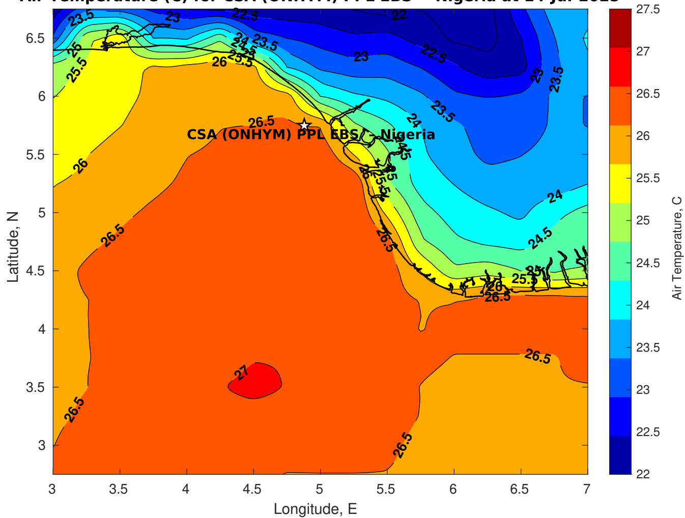
Air Temperature (C) for CSA (ONHYM) PPL EBS - Nigeria at 14-Jul-2025
