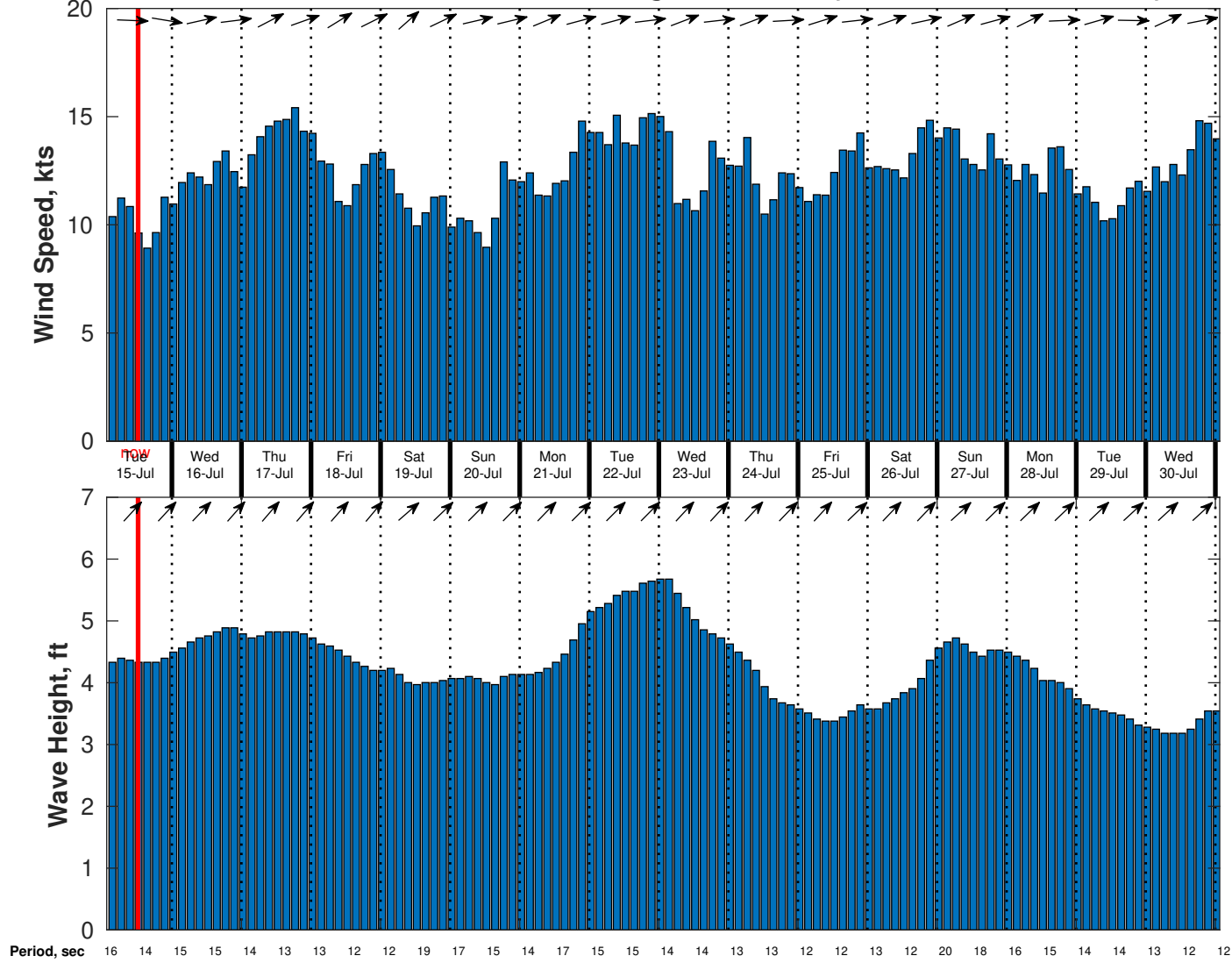
Wind & Wave Forecast for CSA (ONHYM) PPL EBS - Nigeria from 14-Jul-2025 02:00:00 to 30-Jul-2025 02:00:00
