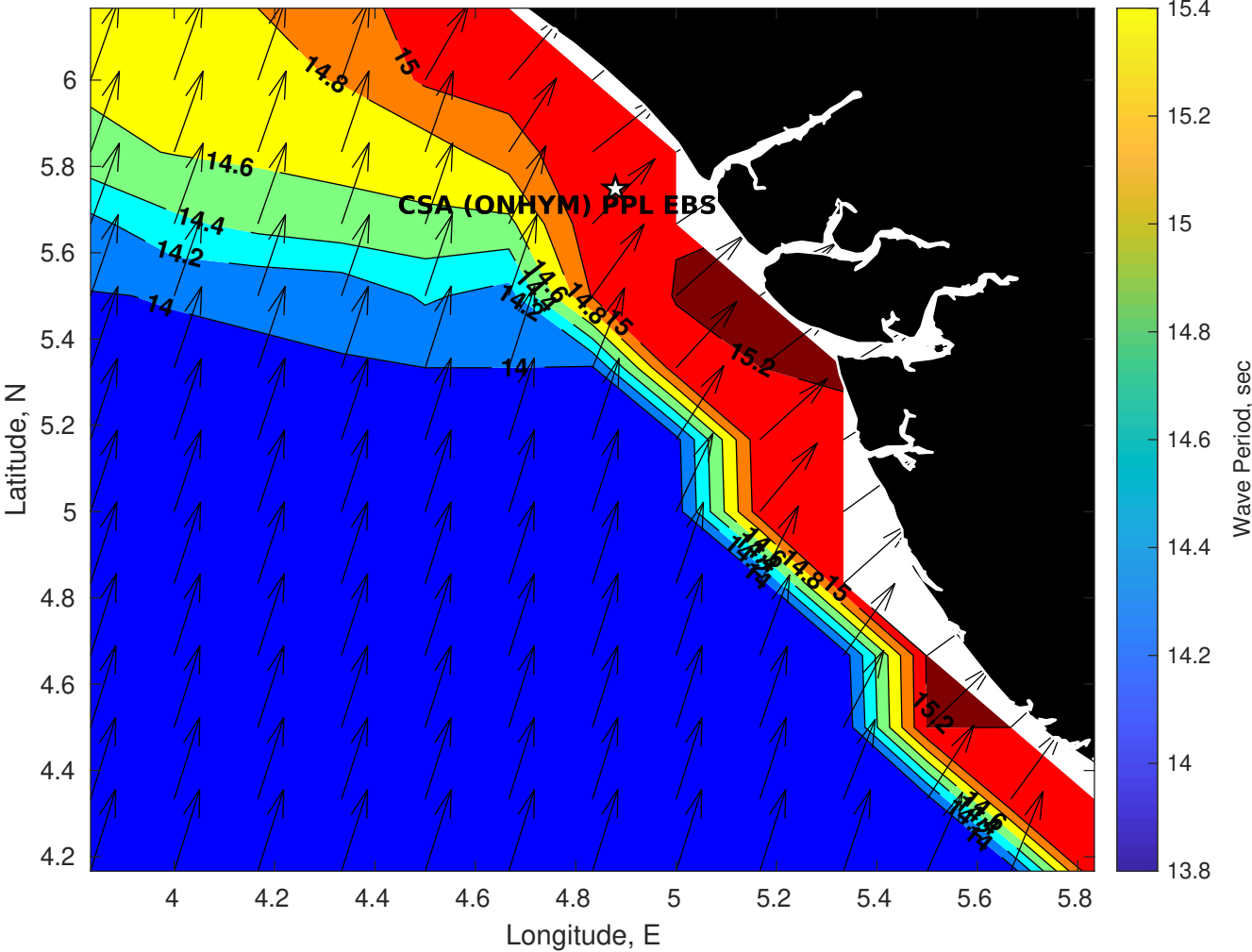
Wave Period (sec) for CSA (ONHYM) PPL EBS - Nigeria at 14-Jul-2025 09:00:00
