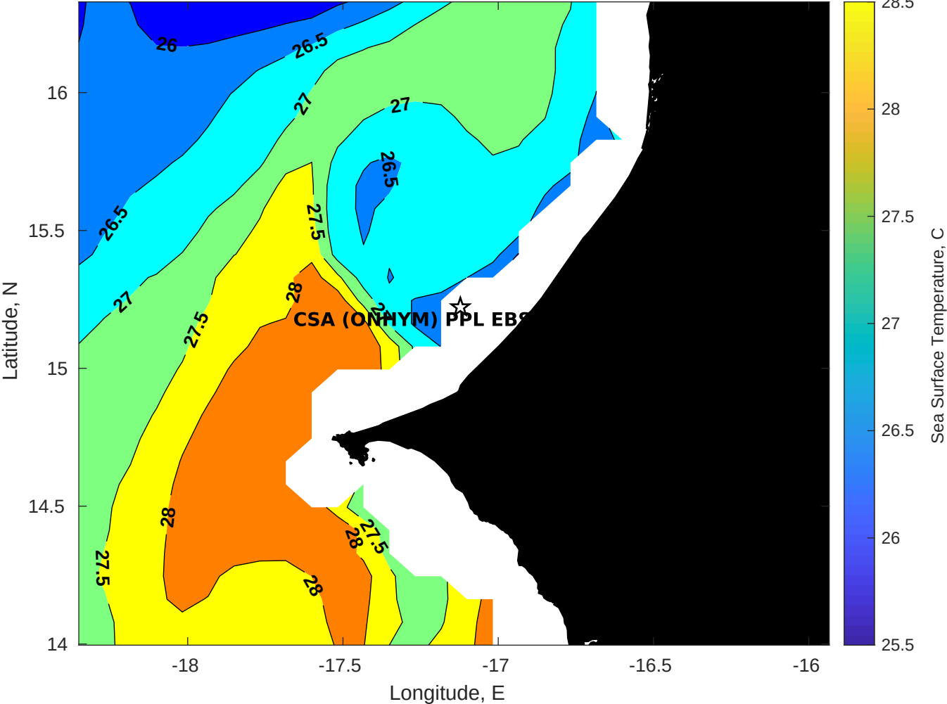
SST for CSA (ONHYM) PPL EBS - Senegal at 13-Jul-2025 00:00:00
