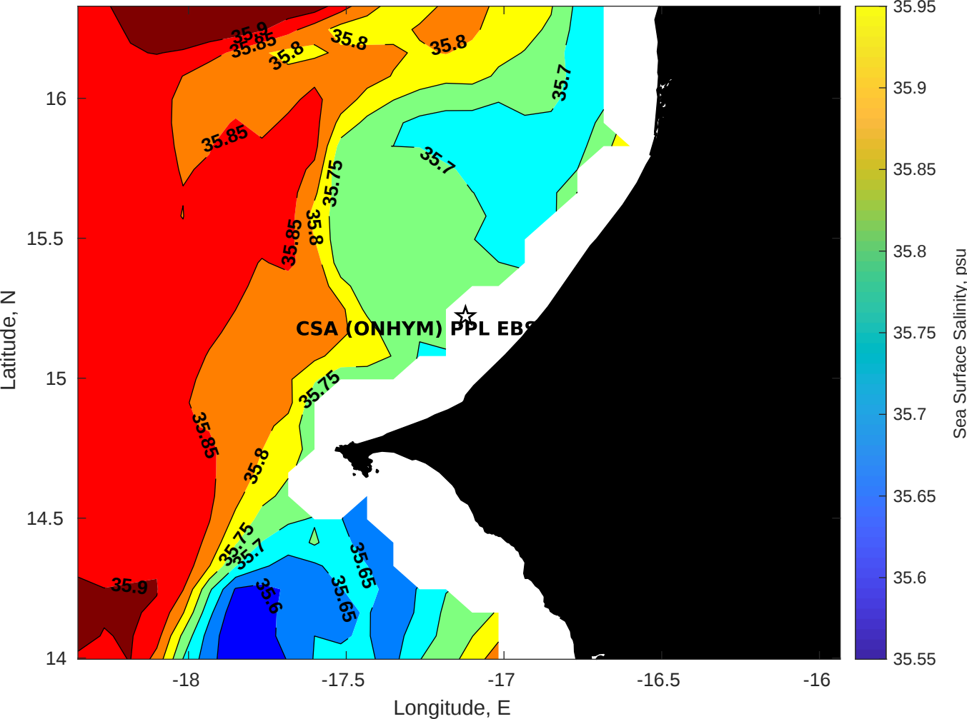
Surface Salinity for CSA (ONHYM) PPL EBS - Senegal at 13-Jul-2025 00:00:00
