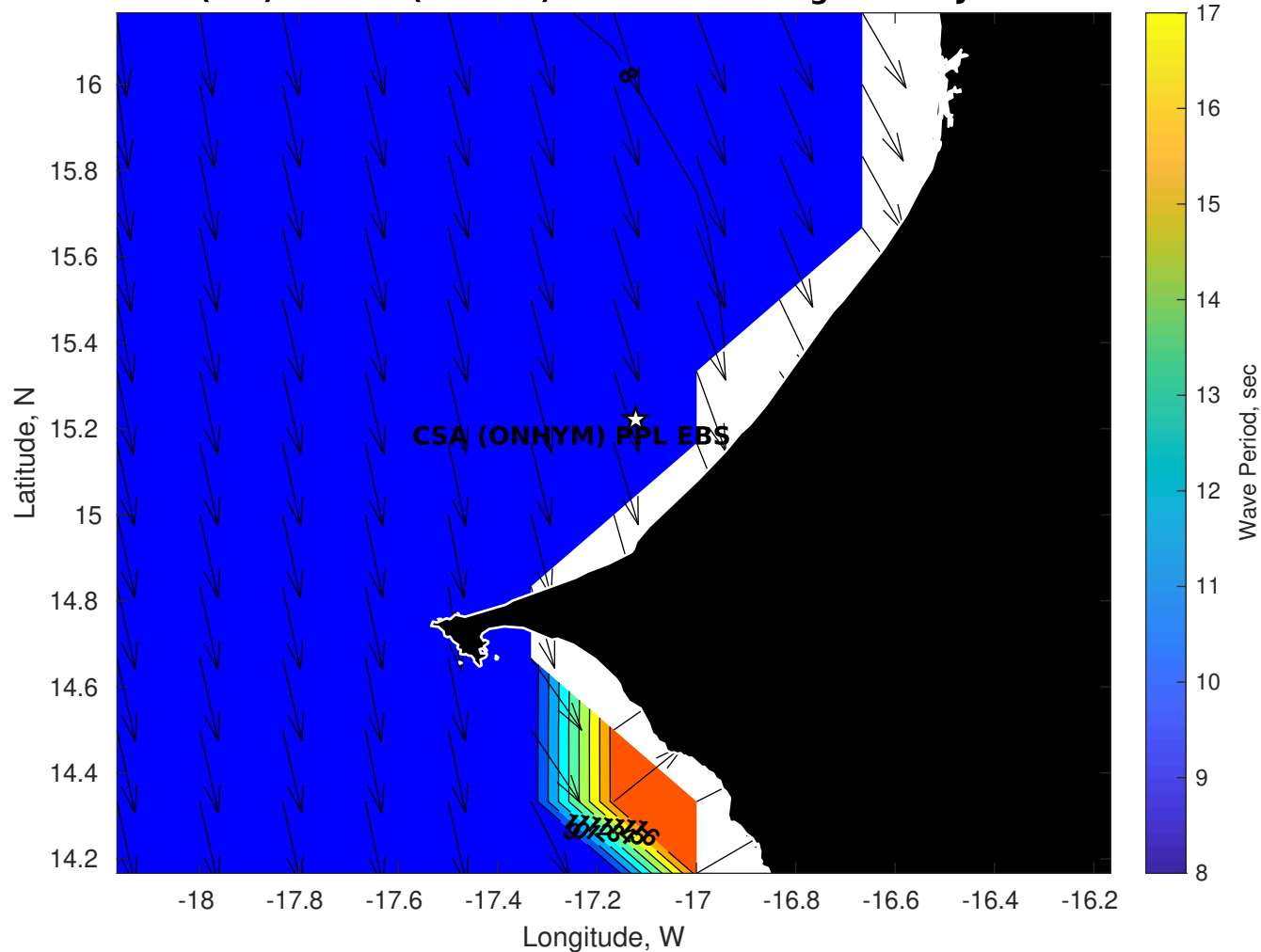
Wave Period (sec) for CSA (ONHYM) PPL EBS - Senegal at 14-Jul-2025 09:00:00
