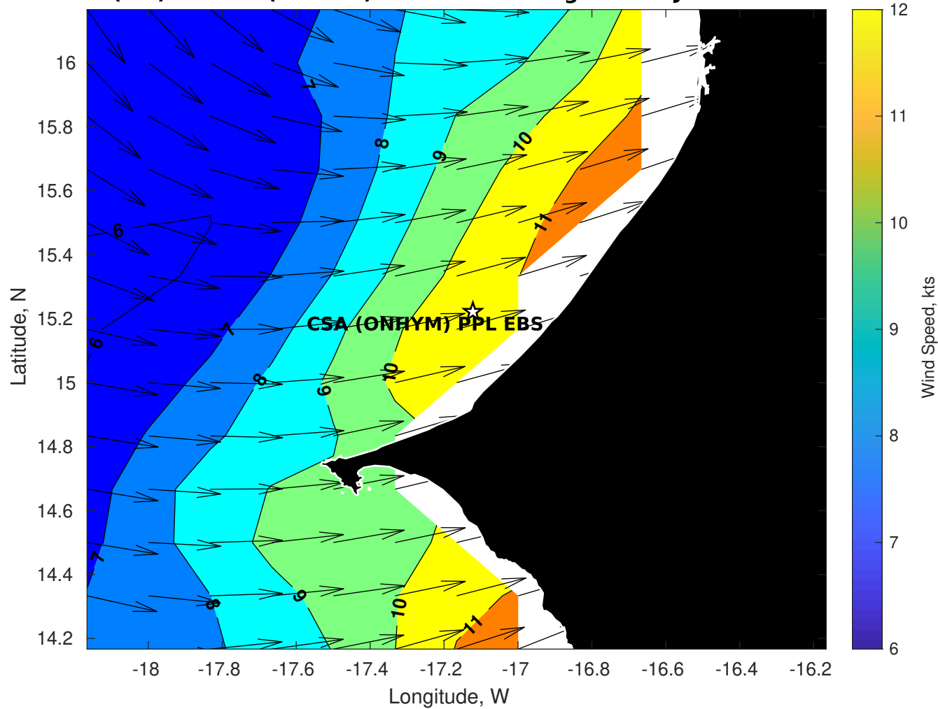
Winds (kts) for CSA (ONHYM) PPL EBS - Senegal at 14-Jul-2025 09:00:00
