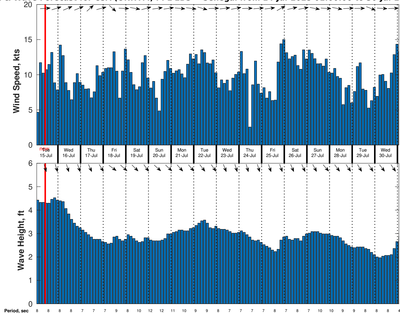
Wind & Wave Forecast for CSA (ONHYM) PPL EBS - Senegal from 14-Jul-2025 01:00:00 to 30-Jul-2025 01:00:00
