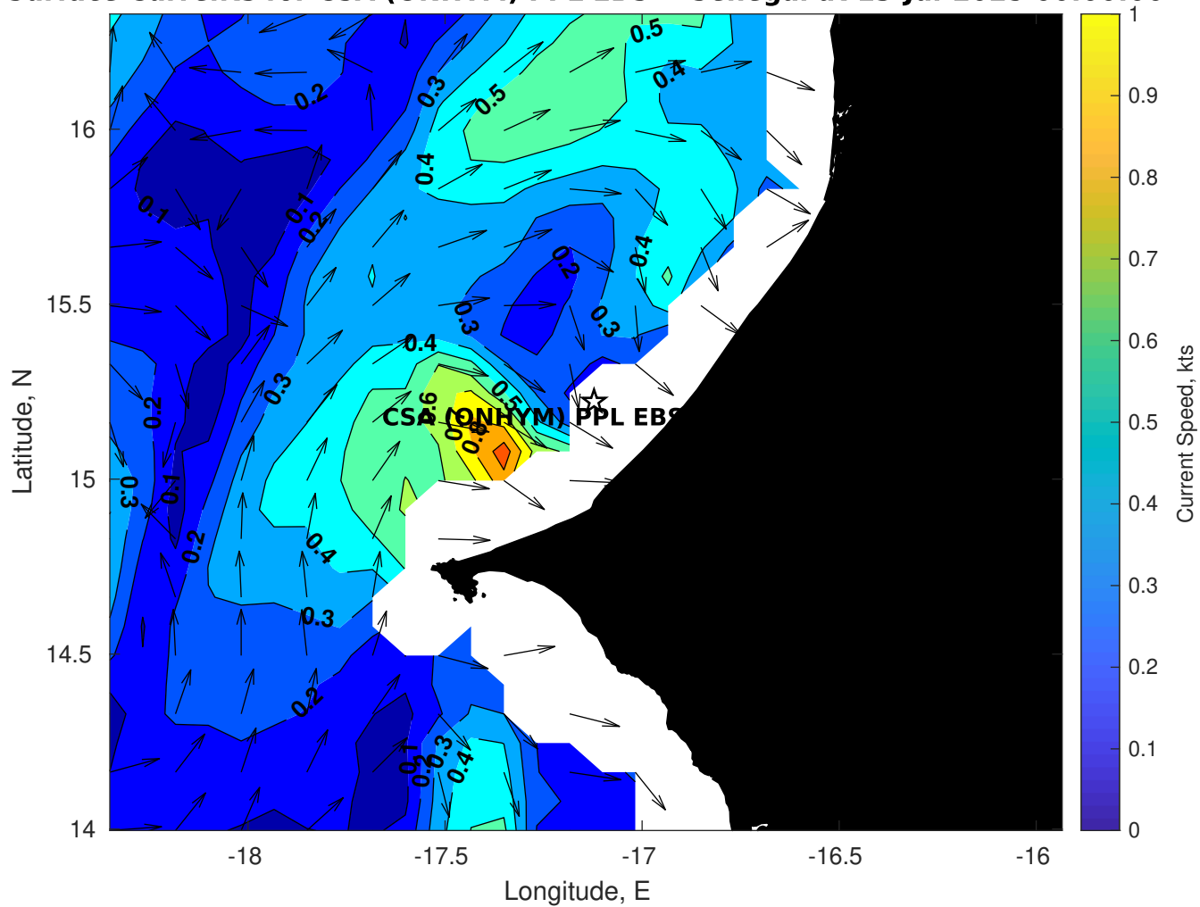
Surface Currents for CSA (ONHYM) PPL EBS - Senegal at 13-Jul-2025 00:00:00
