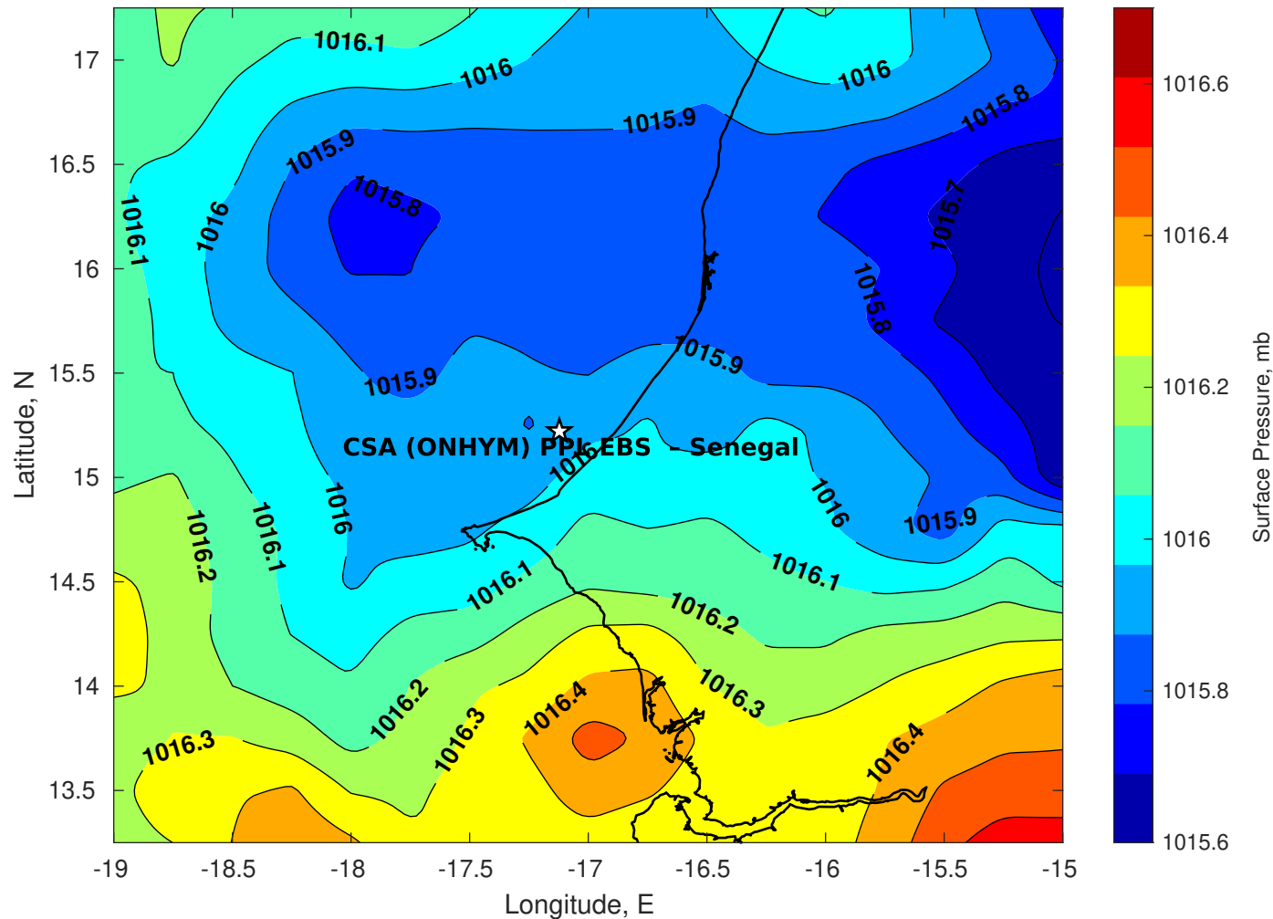
Surface Pressure (mb) for CSA (ONHYM) PPL EBS - Senegal at 16-Jul-2025 00:00:00
