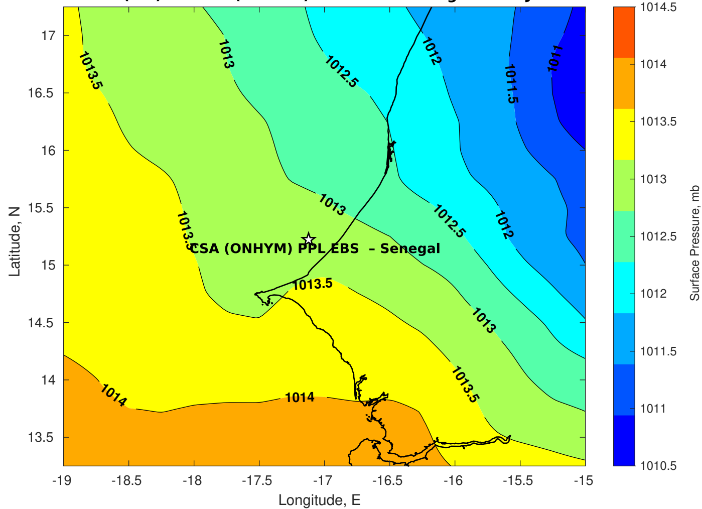
Surface Pressure (mb) for CSA (ONHYM) PPL EBS - Senegal at 14-Jul-2025 00:00:00
