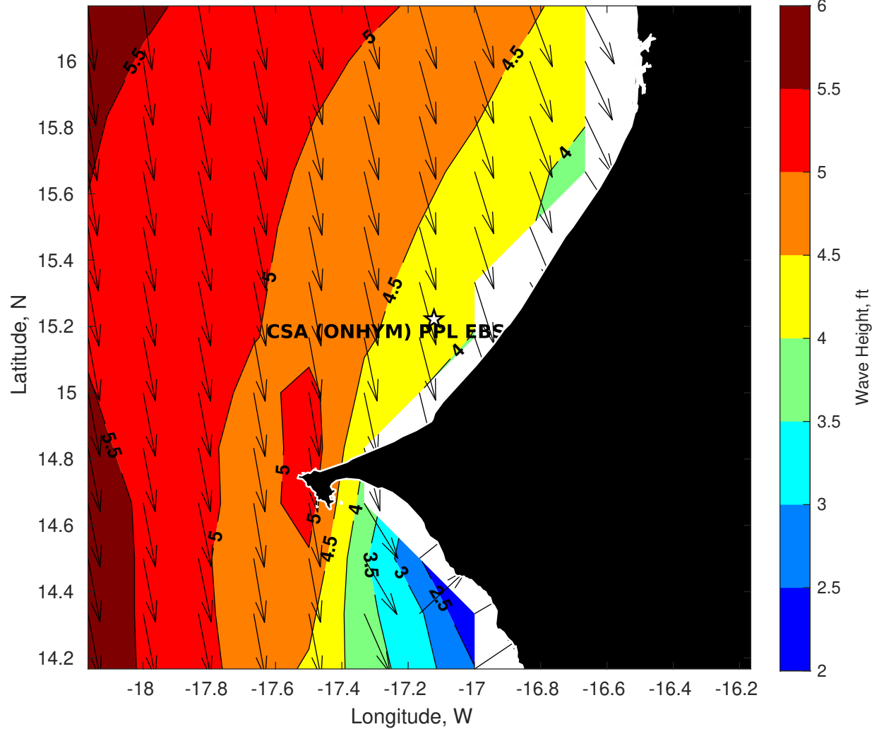
Wave Height (ft) for CSA (ONHYM) PPL EBS - Senegal at 14-Jul-2025 09:00:00
