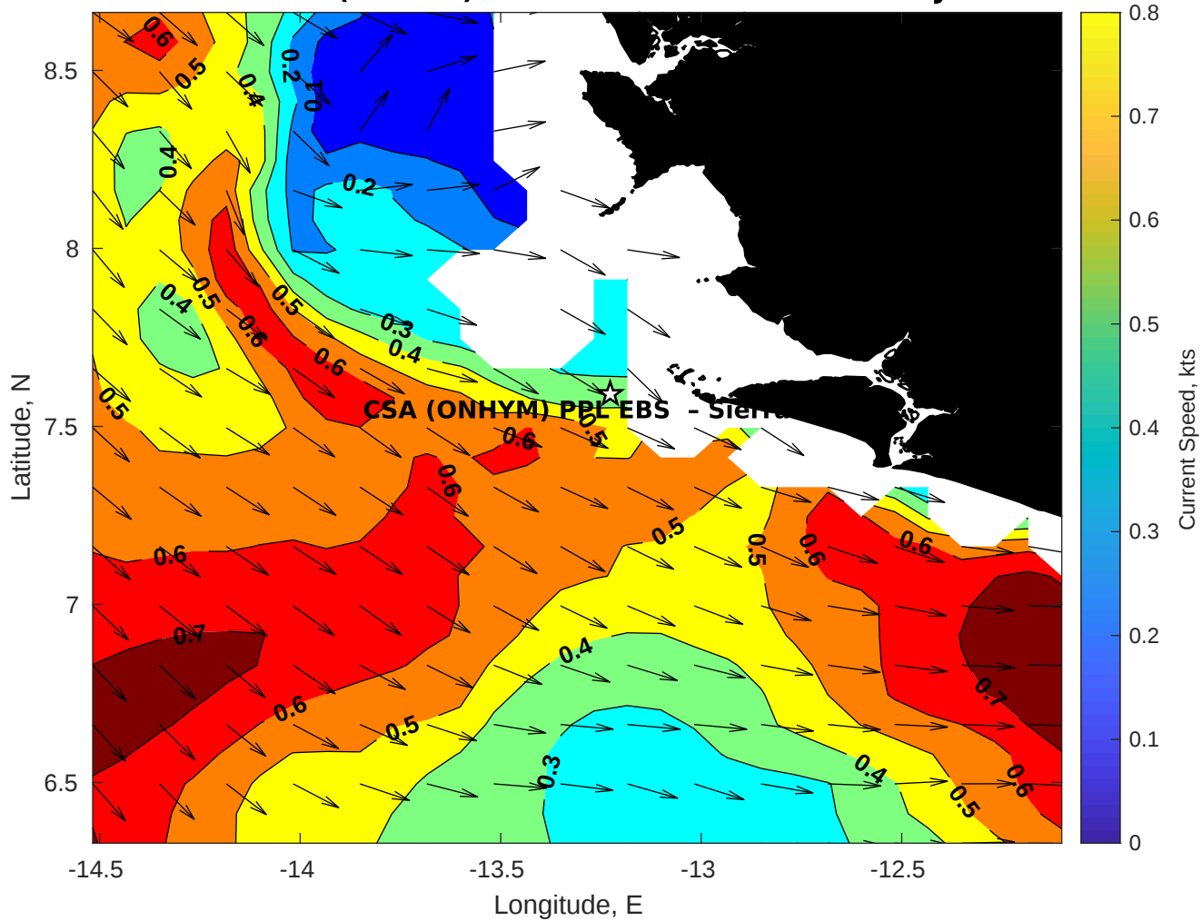
Surface Currents for CSA (ONHYM) PPL EBS - Sierra Leone at 13-Jul-2025 00:00:00
