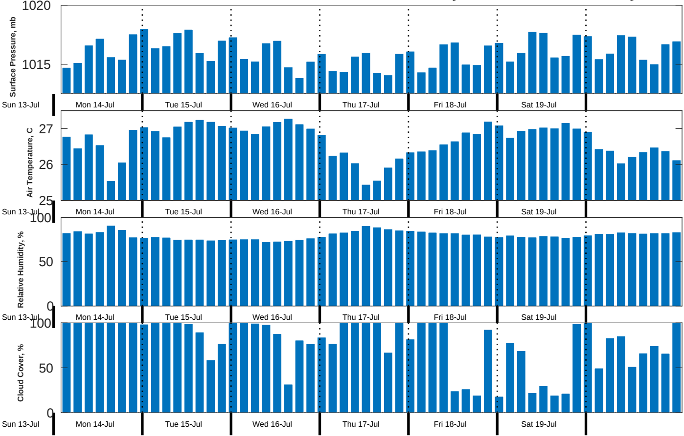
Met Forecast for CSA (ONHYM) PPL EBS - Sierra Leone from 14-Jul-2025 00:00:00 to 21-Jul-2025 00:00:00
