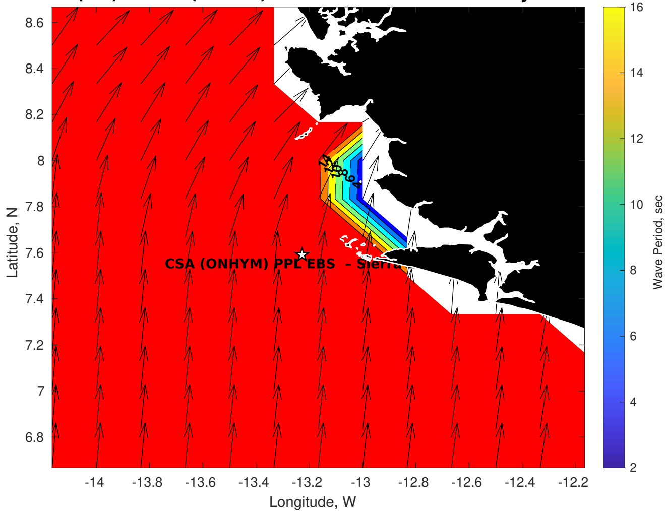
Wave Period (sec) for CSA (ONHYM) PPL EBS - Sierra Leone at 14-Jul-2025 09:00:00
