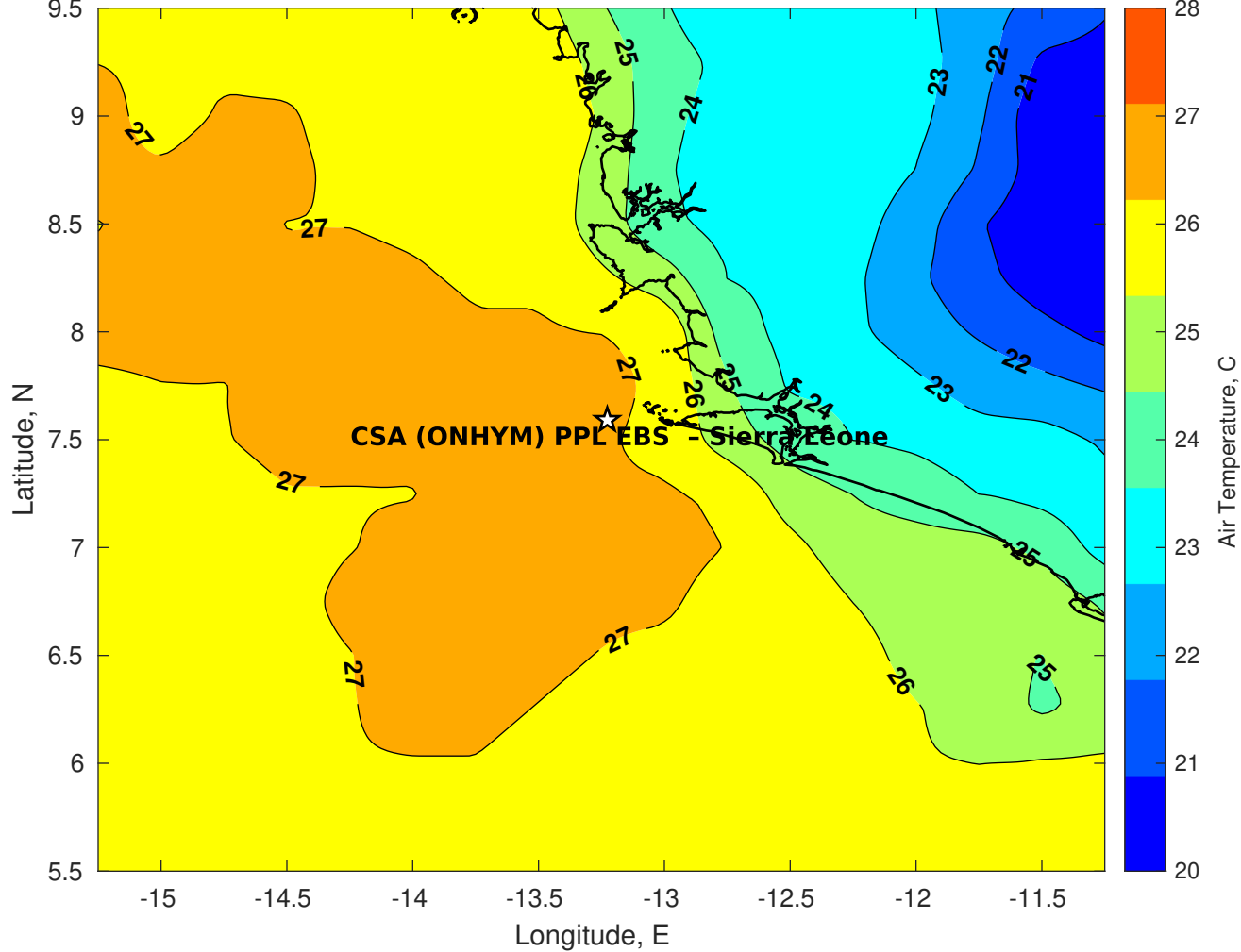
Air Temperature (C) for CSA (ONHYM) PPL EBS - Sierra Leone at 14-Jul-2025
