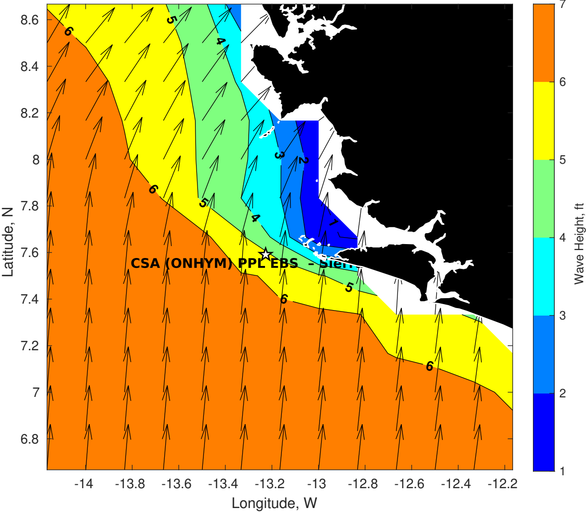
Wave Height (ft) for CSA (ONHYM) PPL EBS - Sierra Leone at 14-Jul-2025 09:00:00
