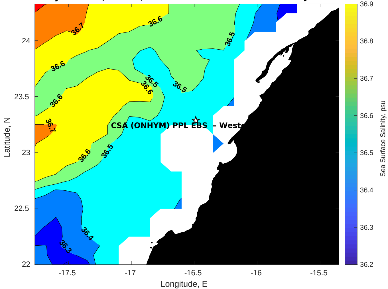
Surface Salinity for CSA (ONHYM) PPL EBS - Western Sahara at 13-Jul-2025 00:00:00
