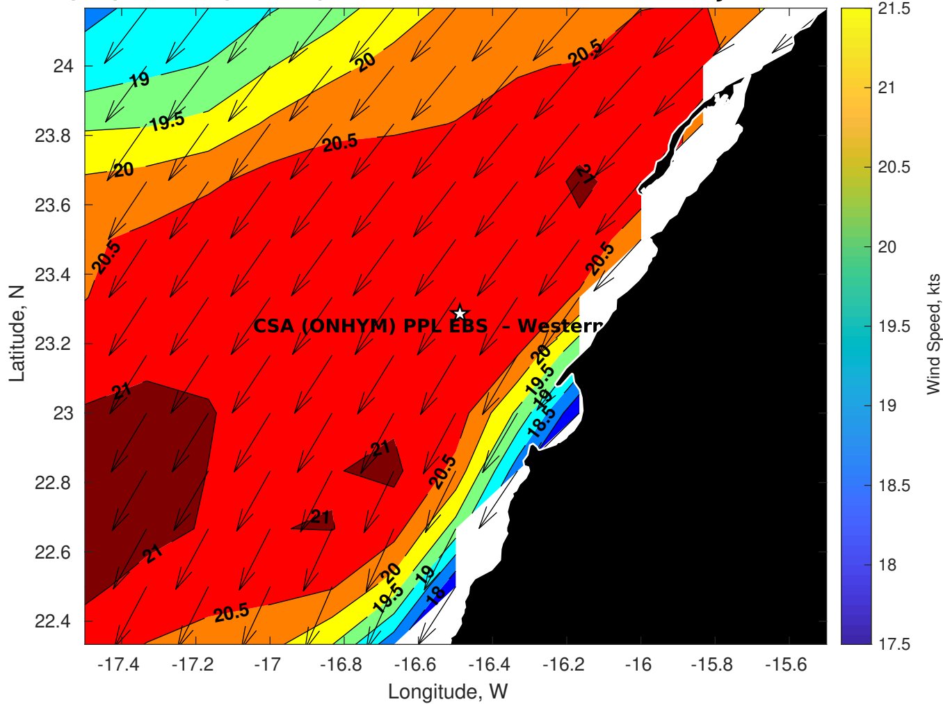
Winds (kts) for CSA (ONHYM) PPL EBS - Western Sahara at 14-Jul-2025 09:00:00
