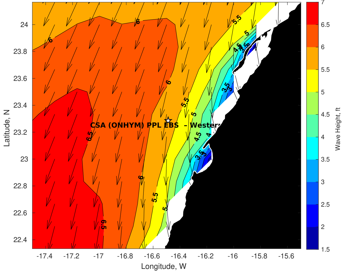
Wave Height (ft) for CSA (ONHYM) PPL EBS - Western Sahara at 14-Jul-2025 09:00:00
