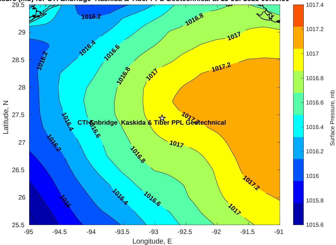
Surface Pressure (mb) for CTI Enbridge Kaskida & Tiber PPL Geotechnical at 15-Jul-2025 00:00:00
