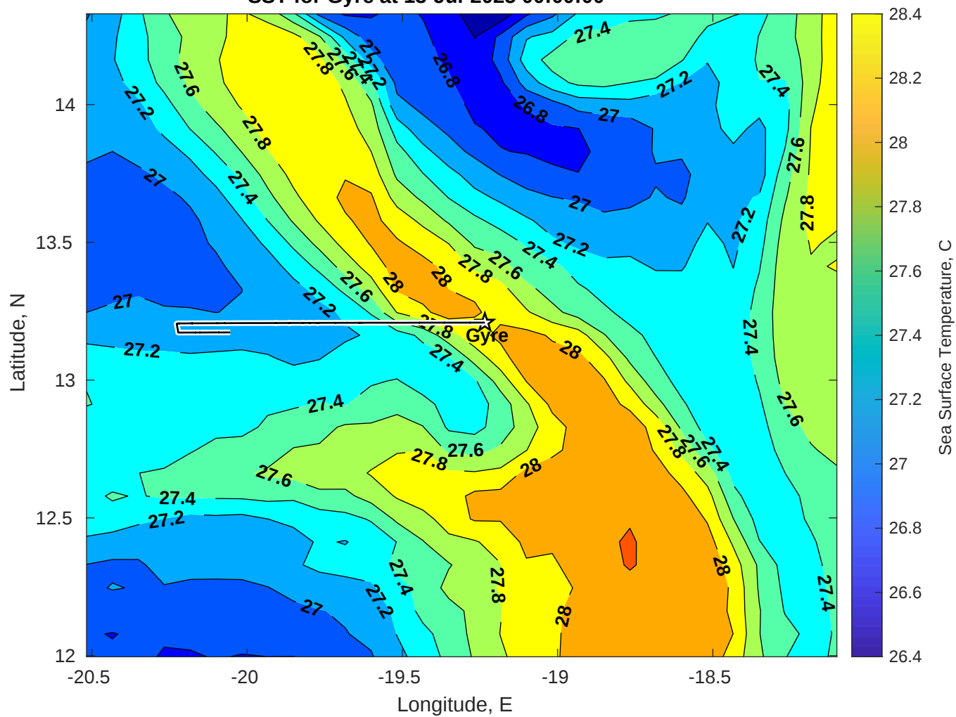
SST for Gyre at 13-Jul-2025 00:00:00
