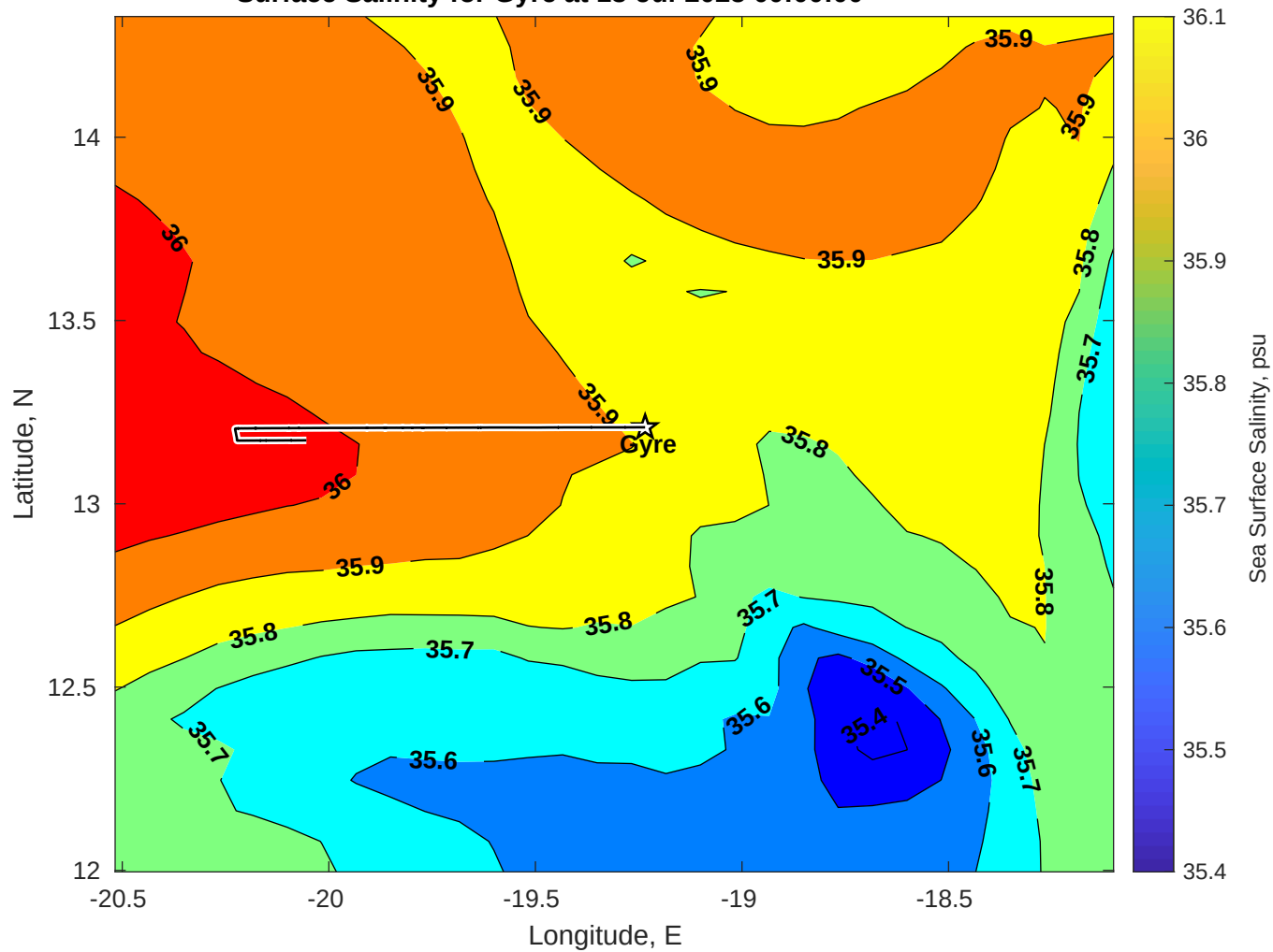
Surface Salinity for Gyre at 13-Jul-2025 00:00:00
