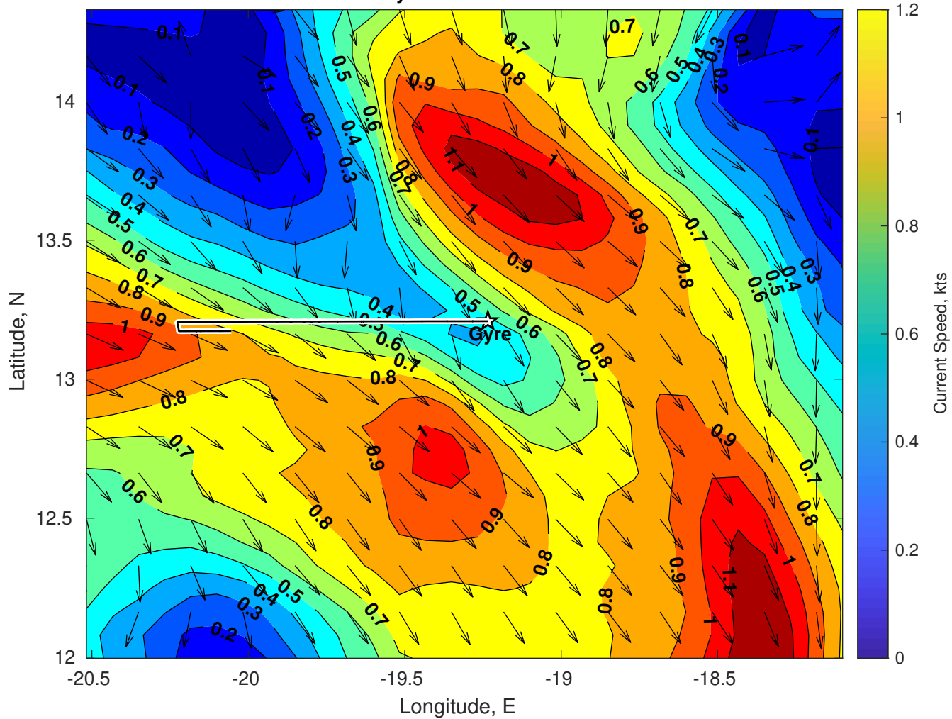
Surface Currents for Gyre at 13-Jul-2025 00:00:00
