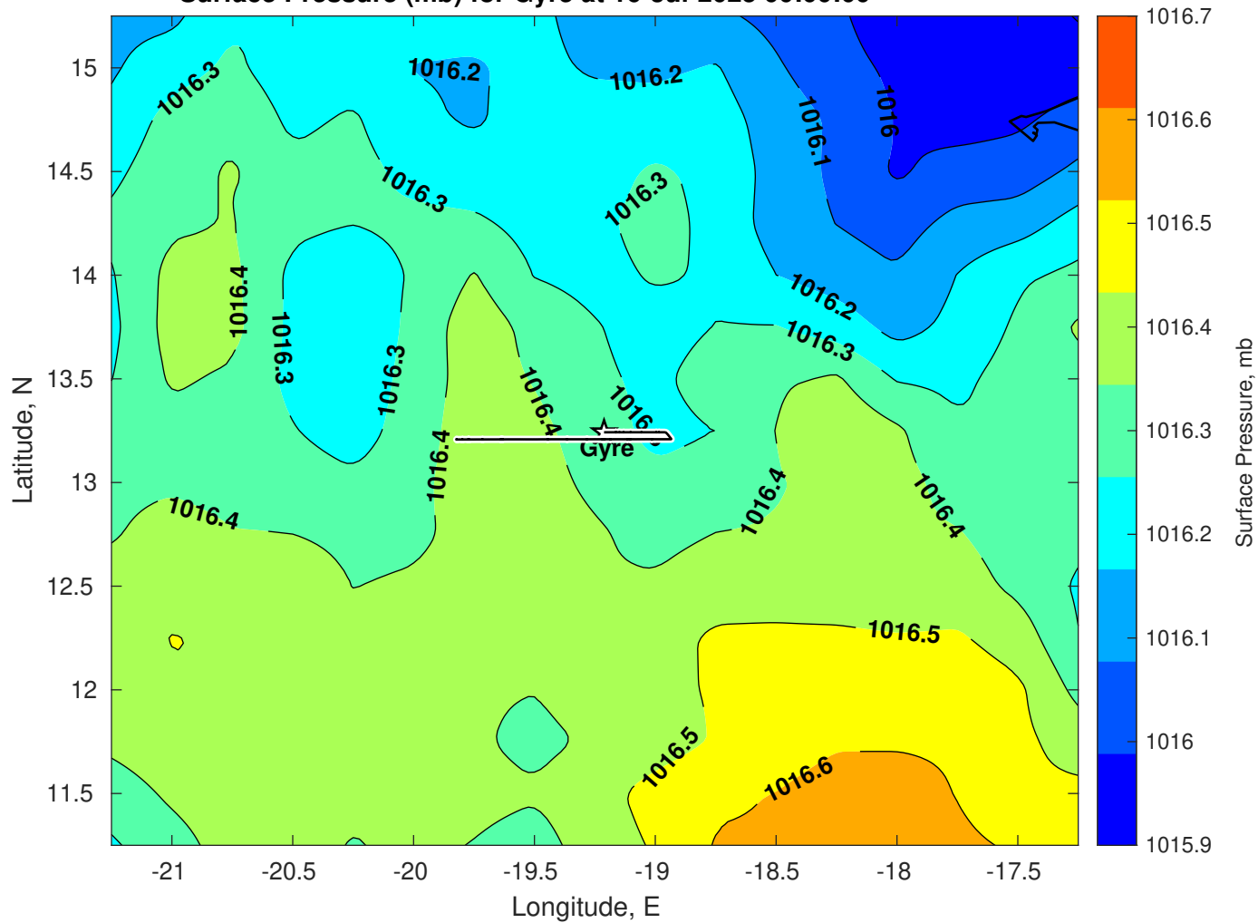
Surface Pressure (mb) for Gyre at 16-Jul-2025 00:00:00
