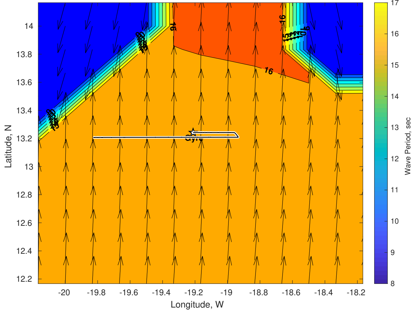
Wave Period (sec) for Gyre at 14-Jul-2025 09:00:00
