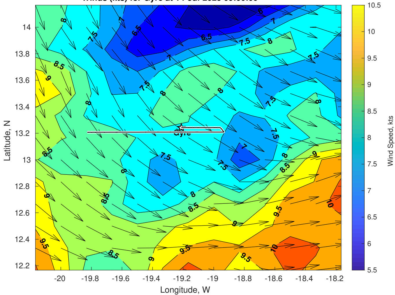
Winds (kts) for Gyre at 14-Jul-2025 09:00:00
