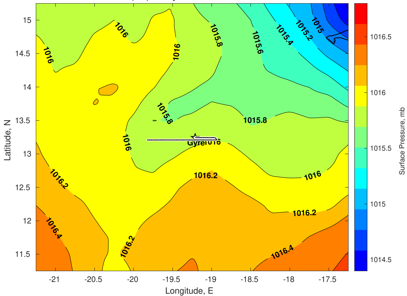
Surface Pressure (mb) for Gyre at 15-Jul-2025 00:00:00
