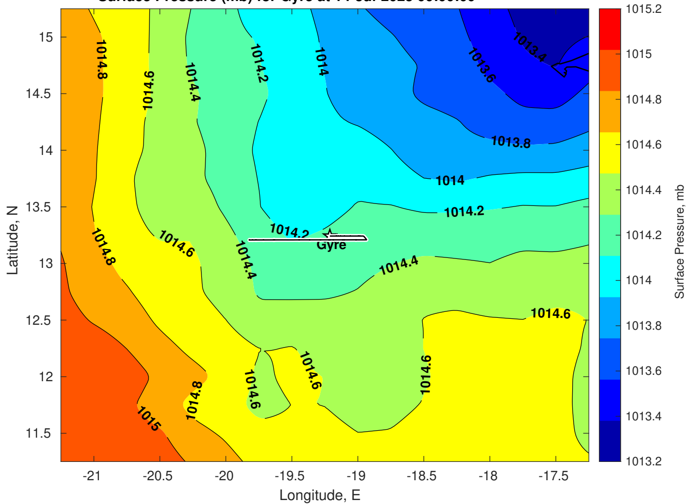
Surface Pressure (mb) for Gyre at 14-Jul-2025 00:00:00
