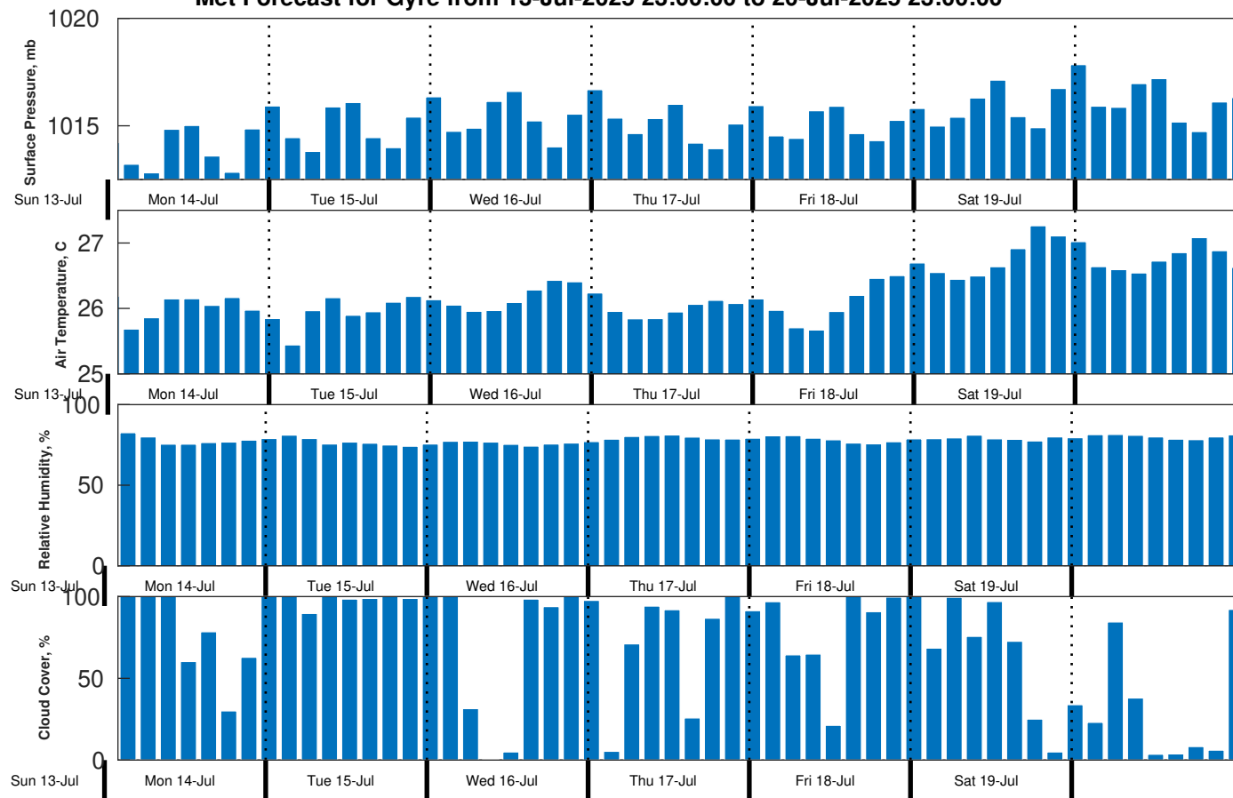
Met Forecast for Gyre from 13-Jul-2025 23:00:00 to 20-Jul-2025 23:00:00
