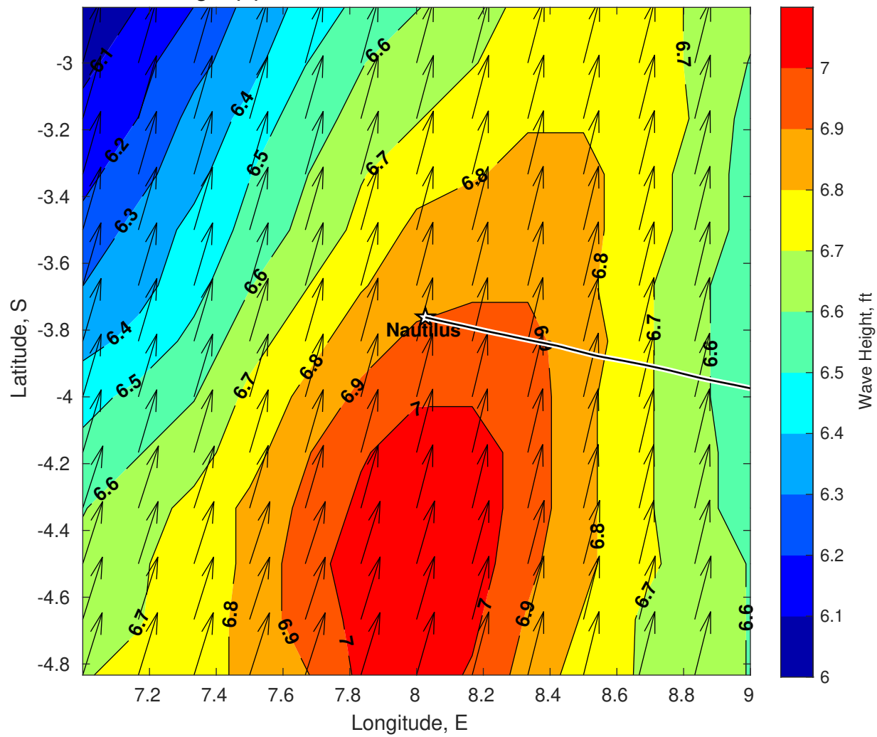
Wave Height (ft) for Nautilus at 14-Jul-2025 09:00:00
