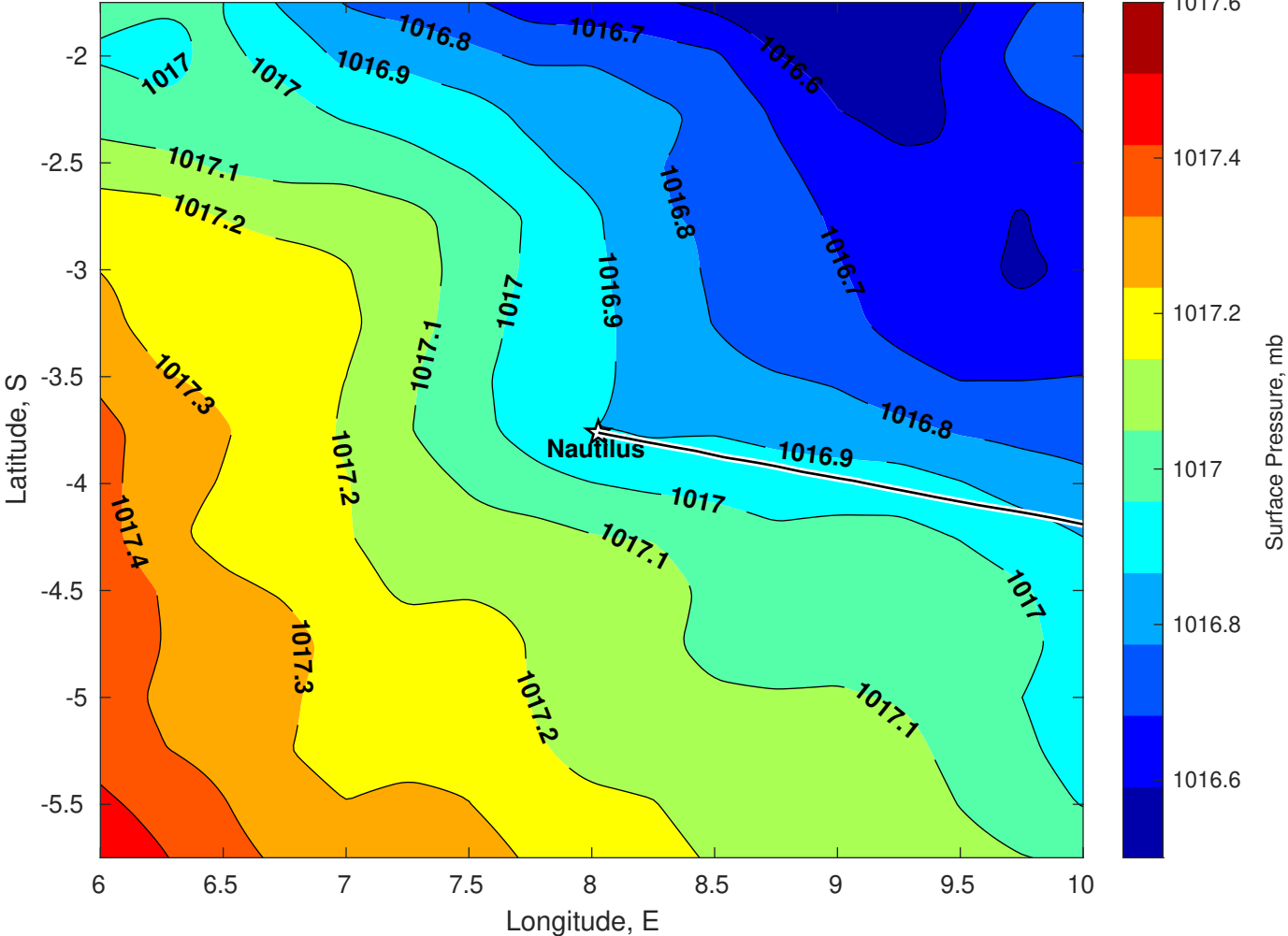
Surface Pressure (mb) for Nautilus at 16-Jul-2025 00:00:00
