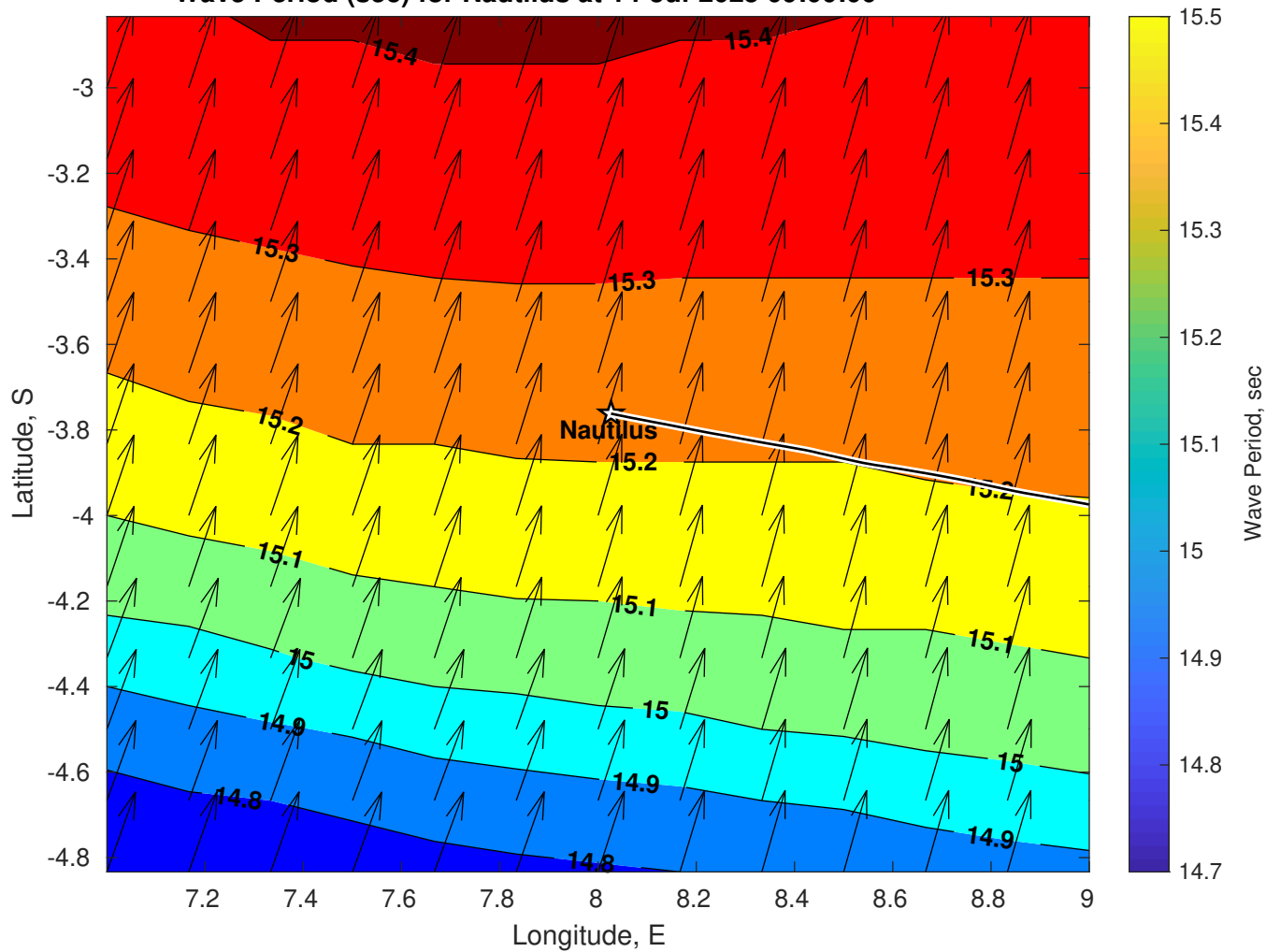
Wave Period (sec) for Nautilus at 14-Jul-2025 09:00:00
