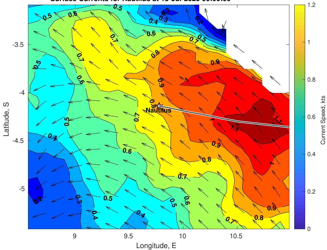
Surface Currents for Nautilus at 13-Jul-2025 00:00:00
