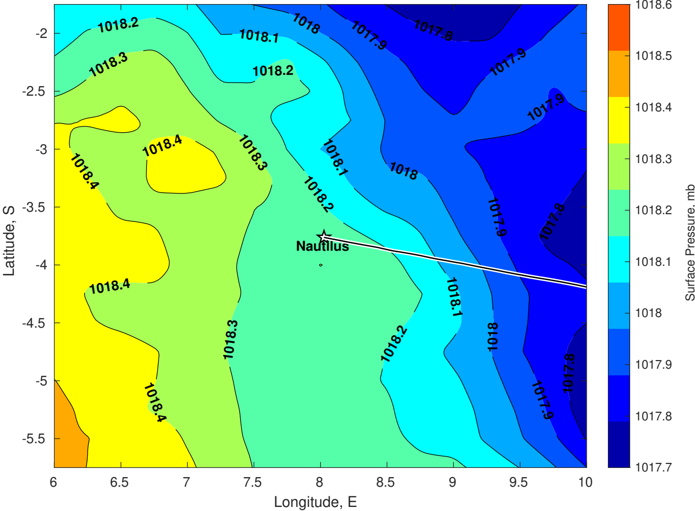
Surface Pressure (mb) for Nautilus at 14-Jul-2025 00:00:00
