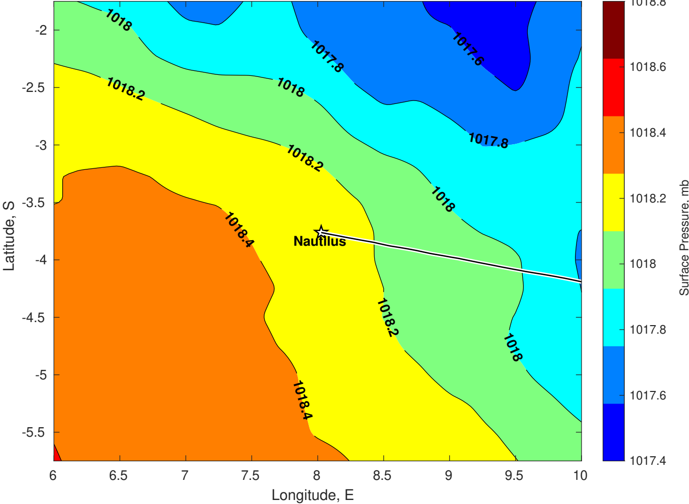
Surface Pressure (mb) for Nautilus at 15-Jul-2025 00:00:00
