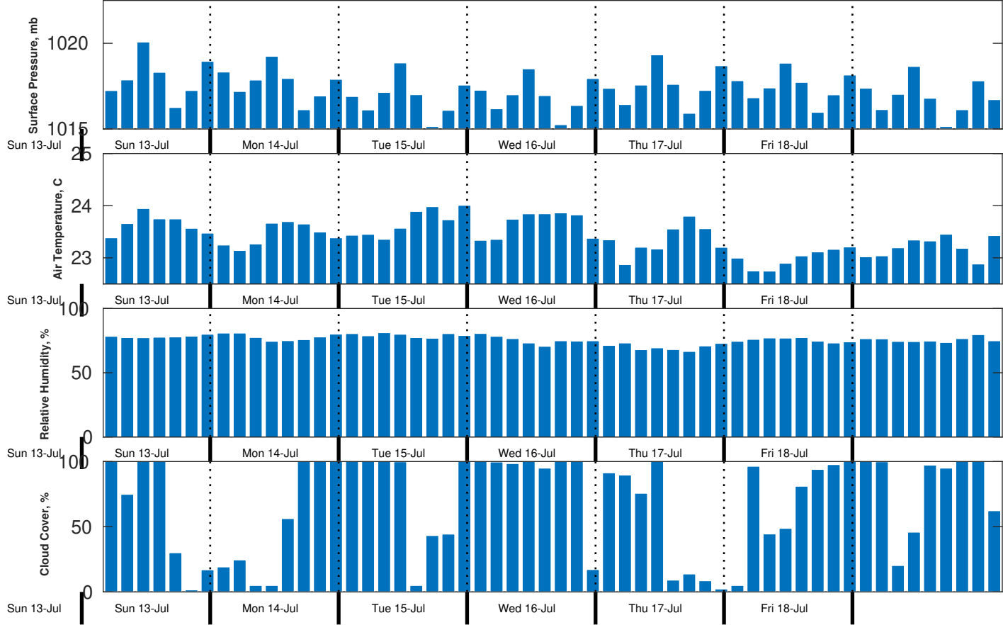
Met Forecast for Nautilus from 14-Jul-2025 00:00:00 to 21-Jul-2025 00:00:00
