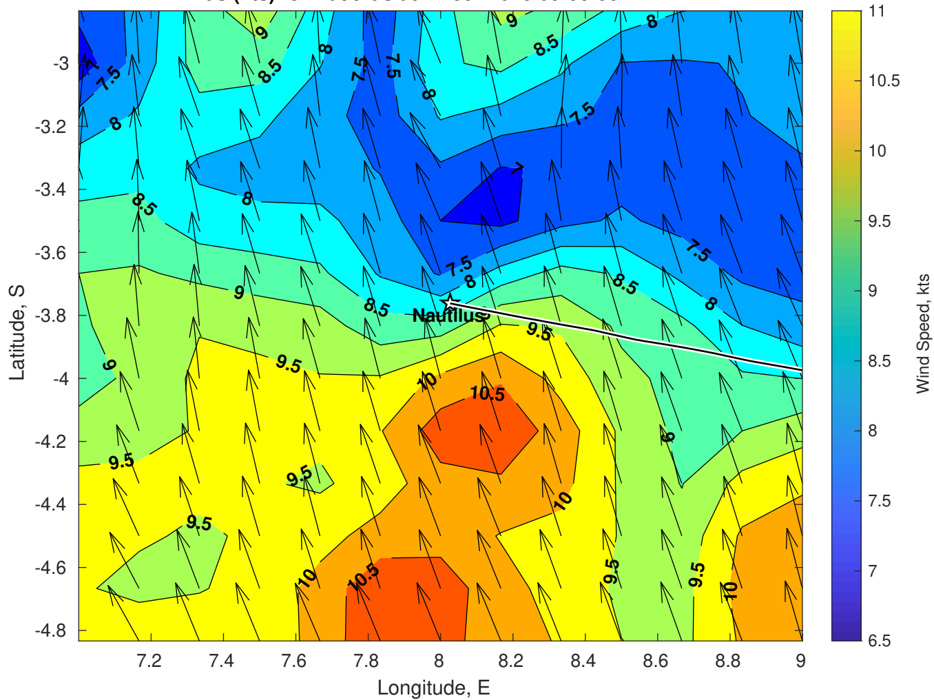
Winds (kts) for Nautilus at 14-Jul-2025 09:00:00
