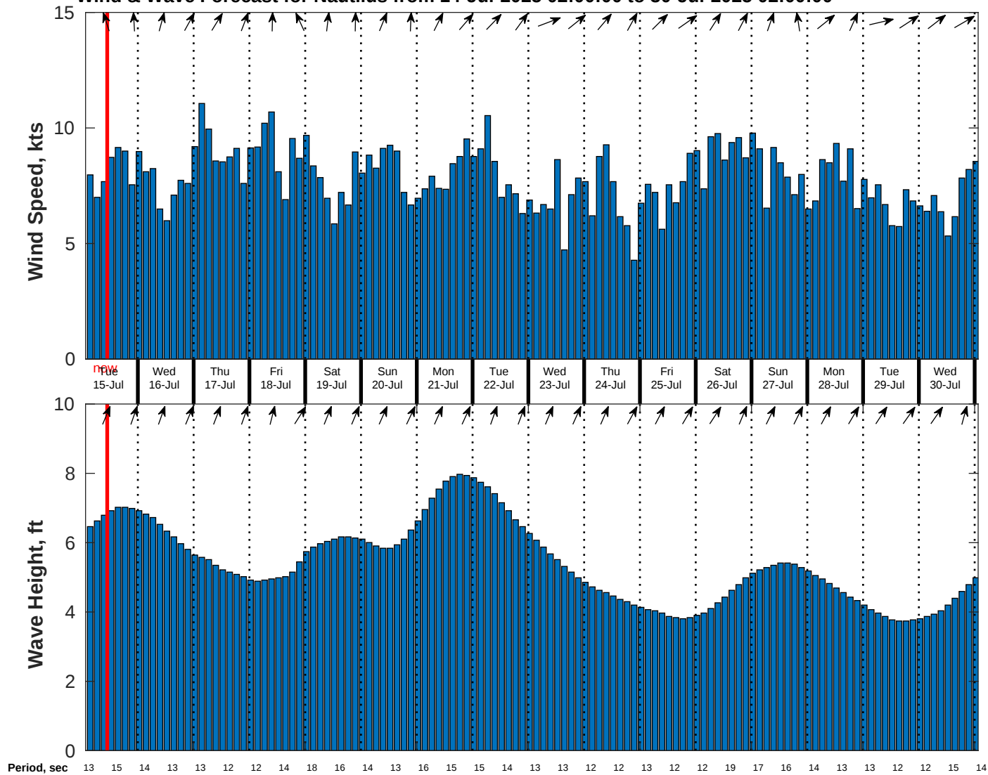
Wind & Wave Forecast for Nautilus from 14-Jul-2025 02:00:00 to 30-Jul-2025 02:00:00
