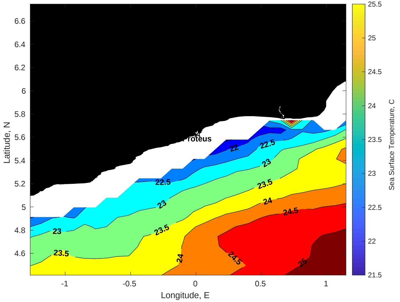
SST for Proteus at 13-Jul-2025 00:00:00
