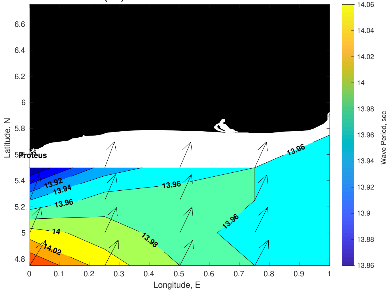
Wave Period (sec) for Proteus at 14-Jul-2025 09:00:00
