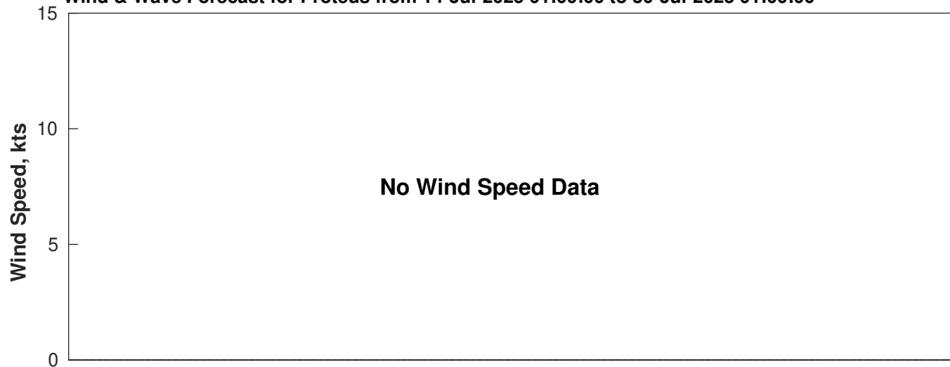
Wind & Wave Forecast for Proteus from 14-Jul-2025 01:00:00 to 30-Jul-2025 01:00:00
