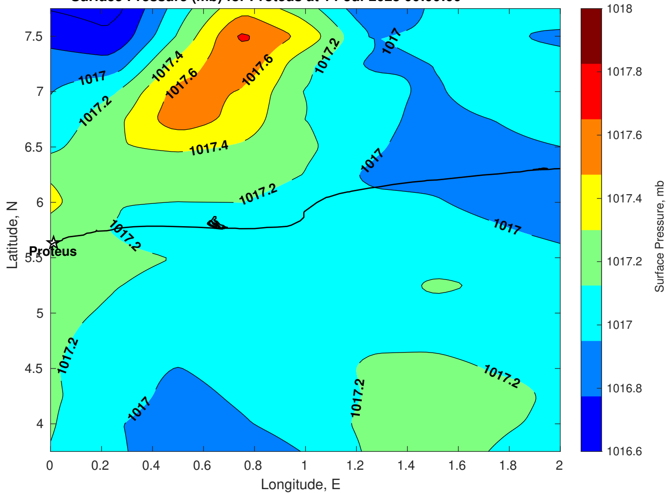
Surface Pressure (mb) for Proteus at 14-Jul-2025 00:00:00
