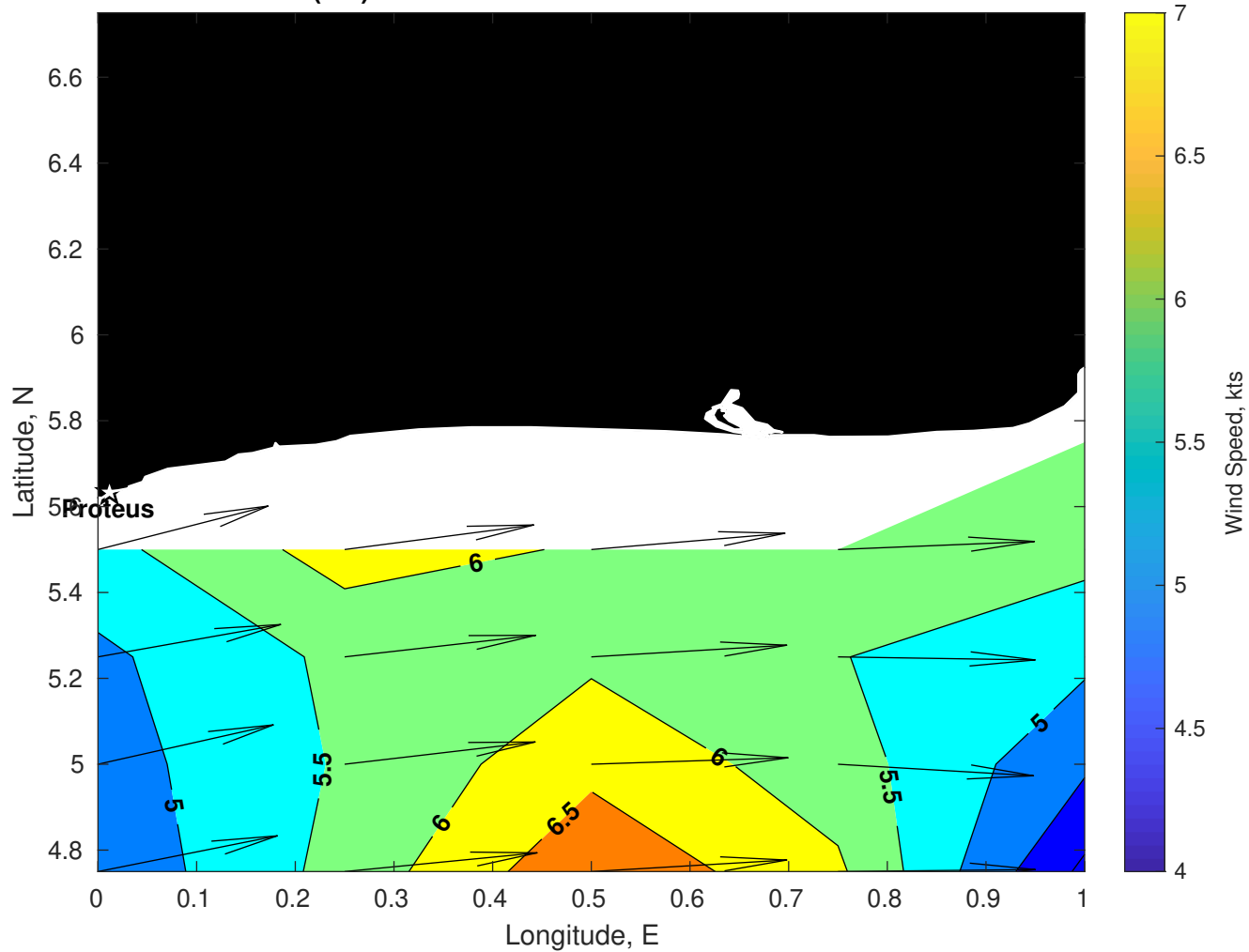
Winds (kts) for Proteus at 14-Jul-2025 09:00:00
