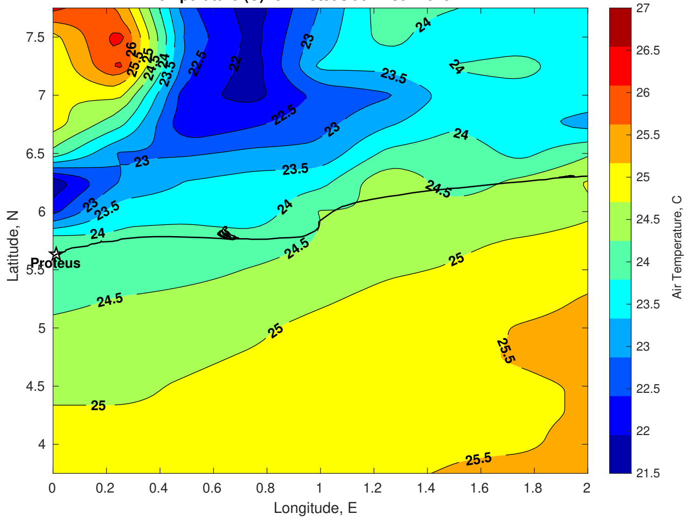
Air Temperature (C) for Proteus at 14-Jul-2025
