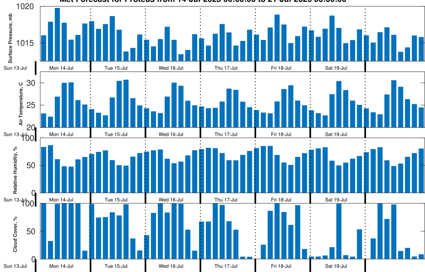
Met Forecast for Proteus from 14-Jul-2025 00:00:00 to 21-Jul-2025 00:00:00
