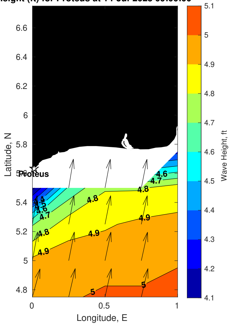
Wave Height (ft) for Proteus at 14-Jul-2025 09:00:00
