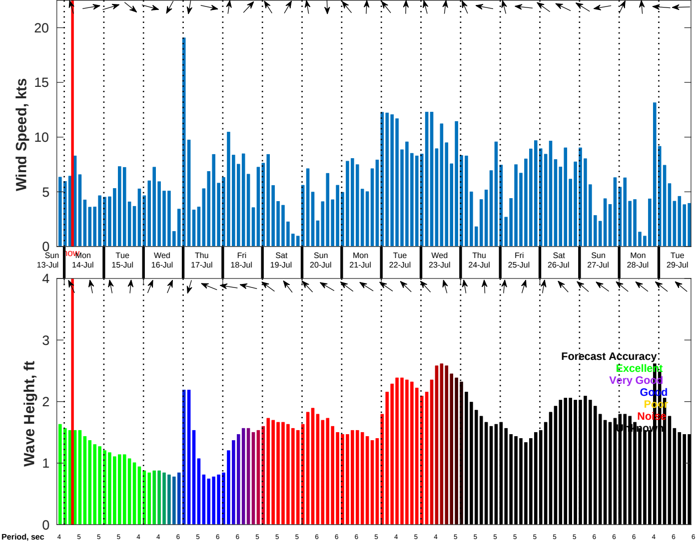
Wind & Wave Forecast for Shell Noches GC19 PPL Geotechnical from 13-Jul-2025 20:00:00 to 29-Jul-2025 20:00:00
