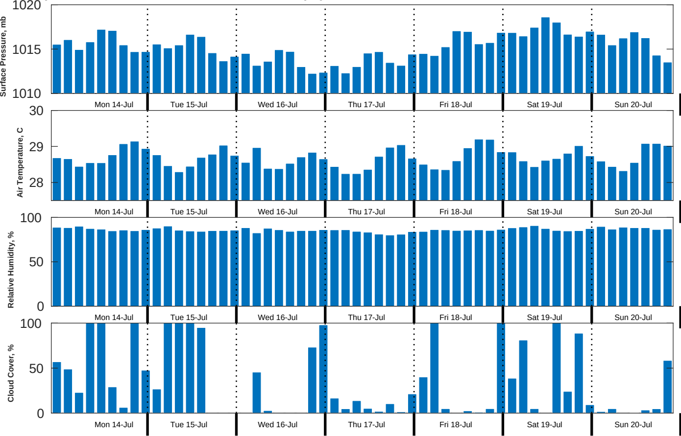
Met Forecast for Tampnet P2378 South Texas Cable Route Geophysical from 14-Jul-2025 00:00:00 to 21-Jul-2025 00:00:00
