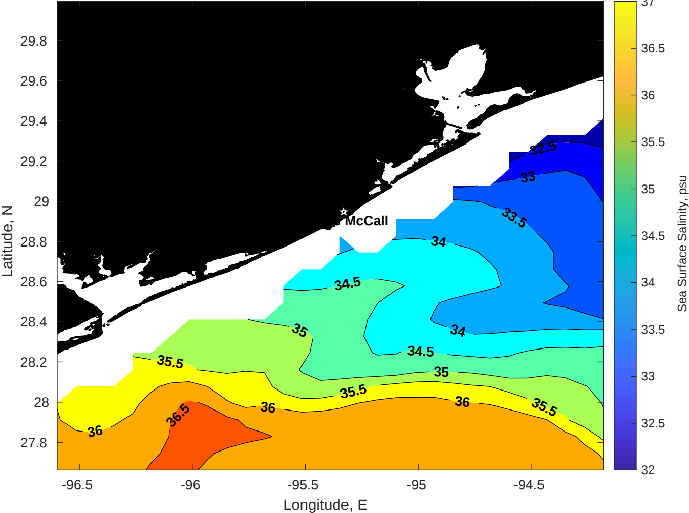
Surface Salinity for Brooks McCall at 14-Jul-2025 00:00:00
