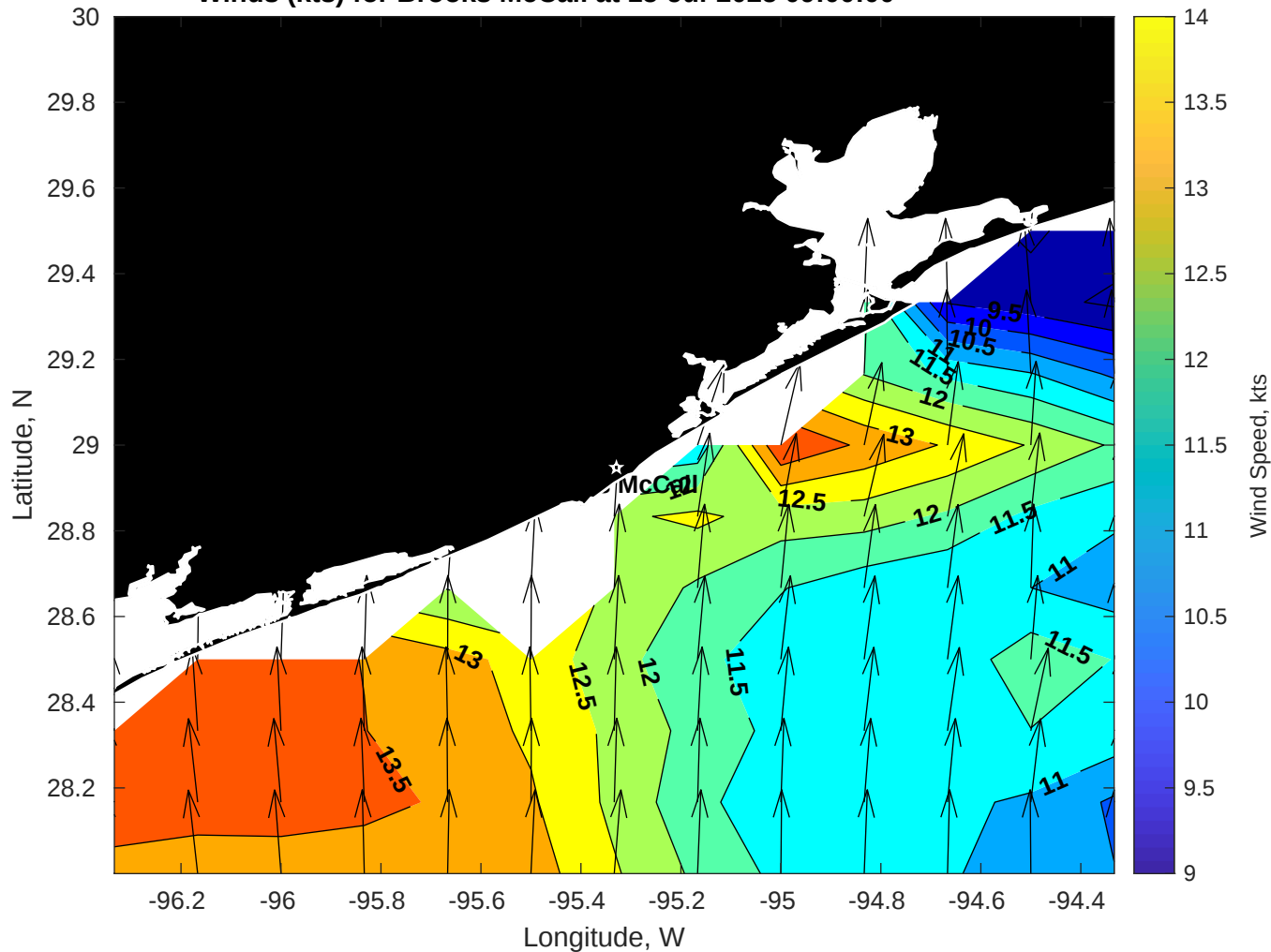
Winds (kts) for Brooks McCall at 15-Jul-2025 09:00:00
