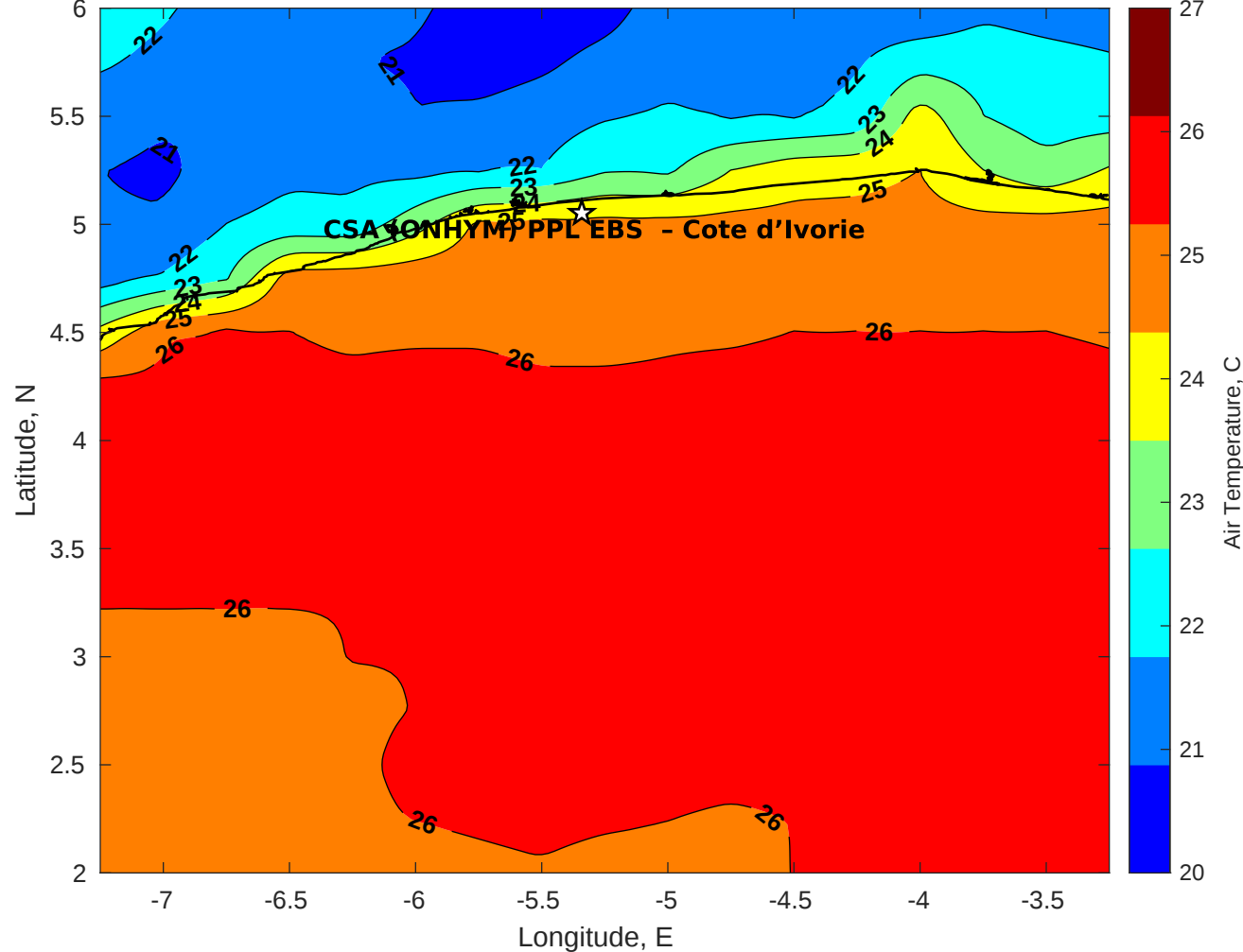
Air Temperature (C) for CSA (ONHYM) PPL EBS - Cote d'Ivoire at 15-Jul-2025
