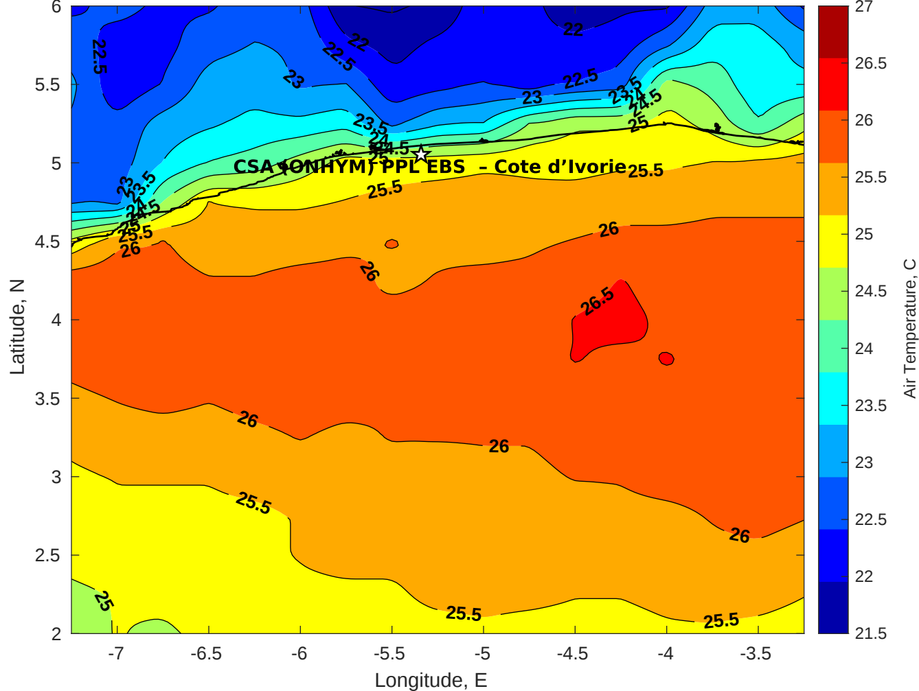
Air Temperature (C) for CSA (ONHYM) PPL EBS - Cote d'Ivoire at 15-Jul-2025
