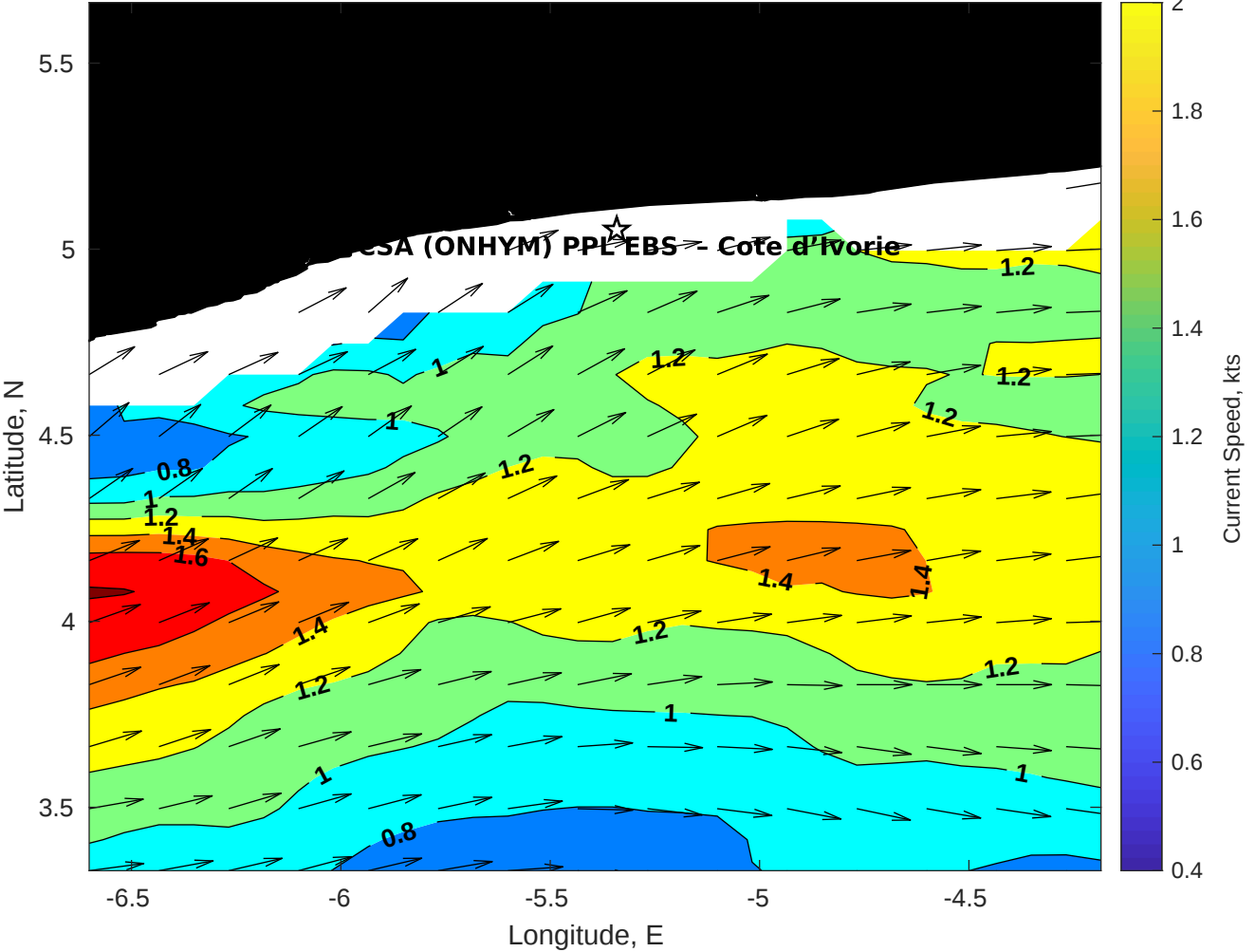
Surface Currents for CSA (ONHYM) PPL EBS - Cote d'Ivoire at 14-Jul-2025 00:00:00
