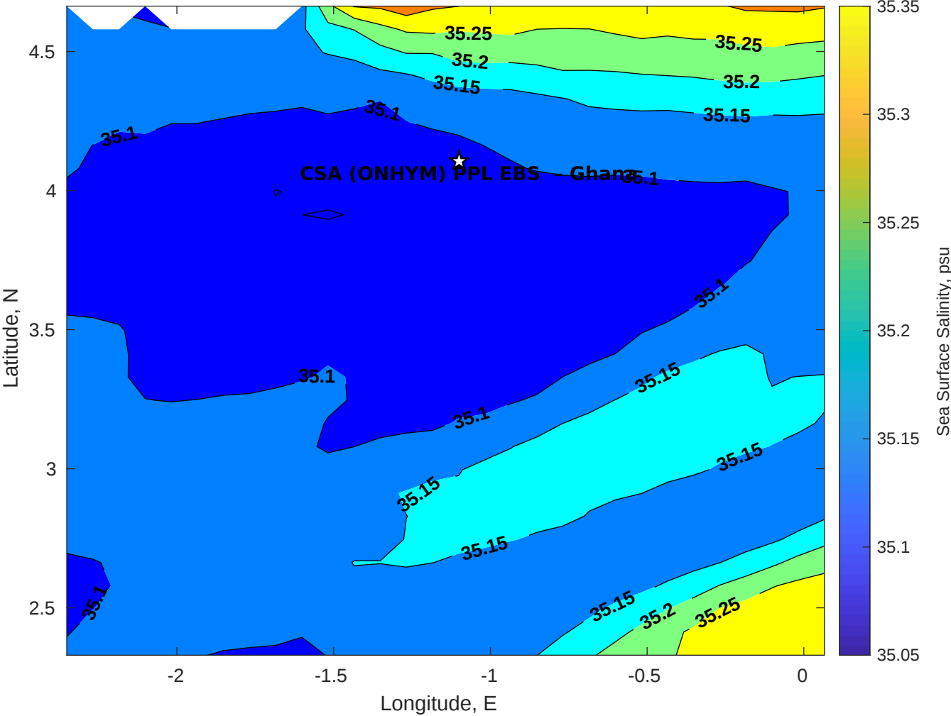
Surface Salinity for CSA (ONHYM) PPL EBS - Ghana at 14-Jul-2025 00:00:00
