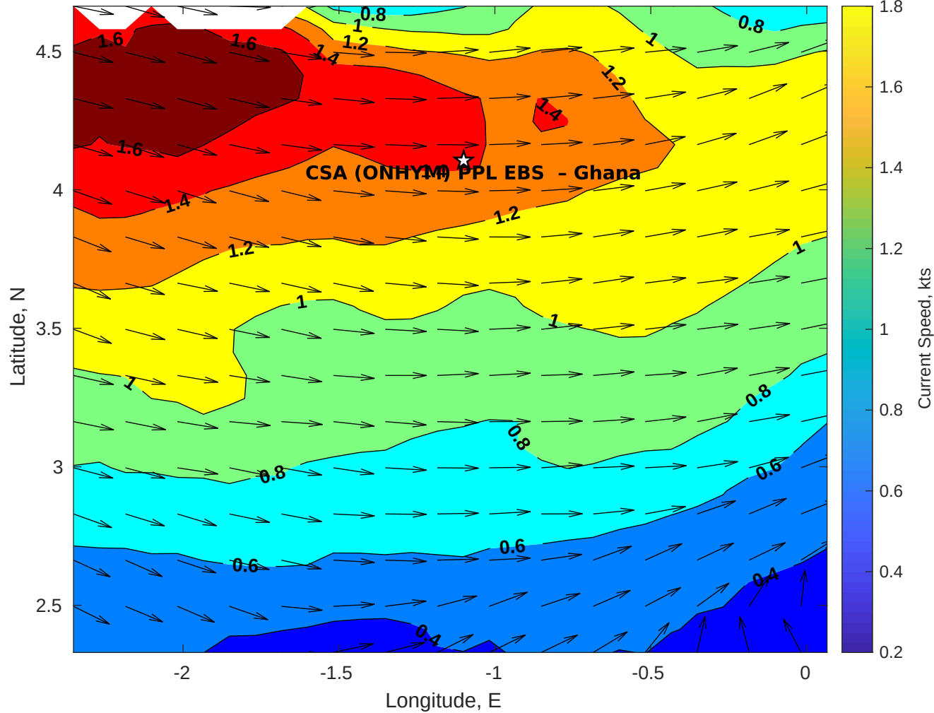
Surface Currents for CSA (ONHYM) PPL EBS - Ghana at 14-Jul-2025 00:00:00
