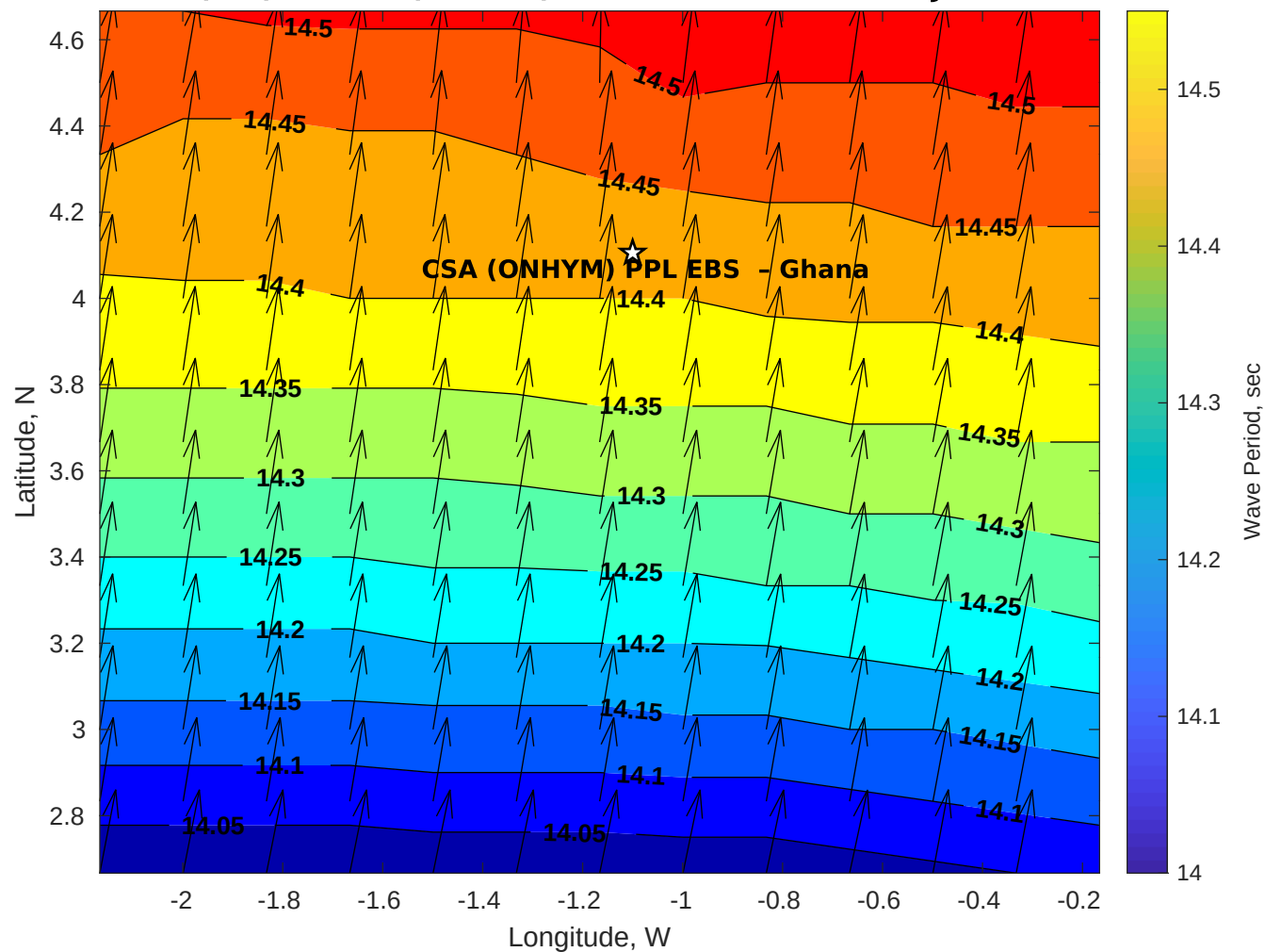
Wave Period (sec) for CSA (ONHYM) PPL EBS - Ghana at 15-Jul-2025 09:00:00
