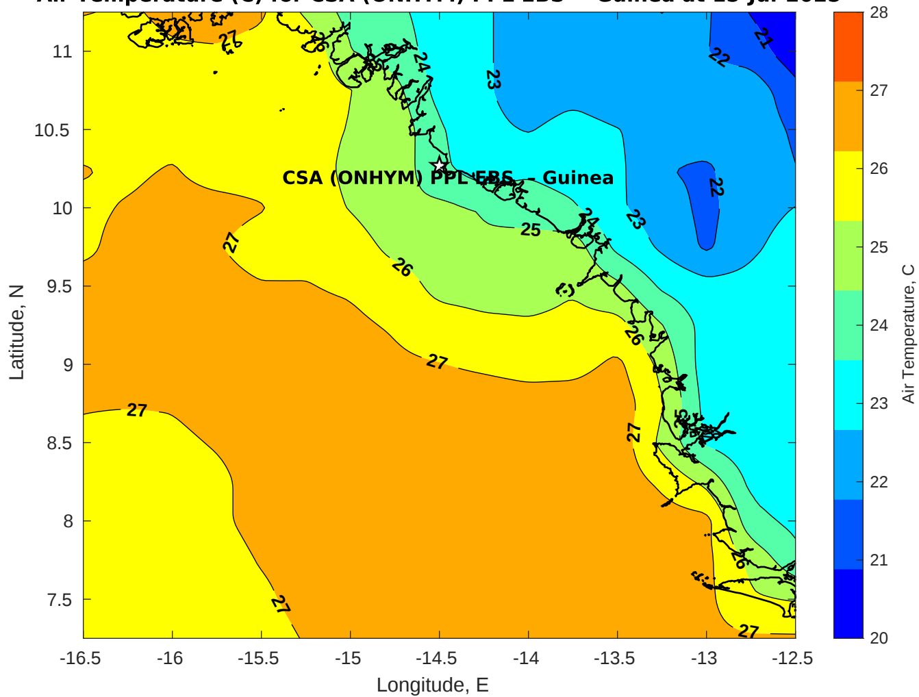
Air Temperature (C) for CSA (ONHYM) PPL EBS - Guinea at 15-Jul-2025
