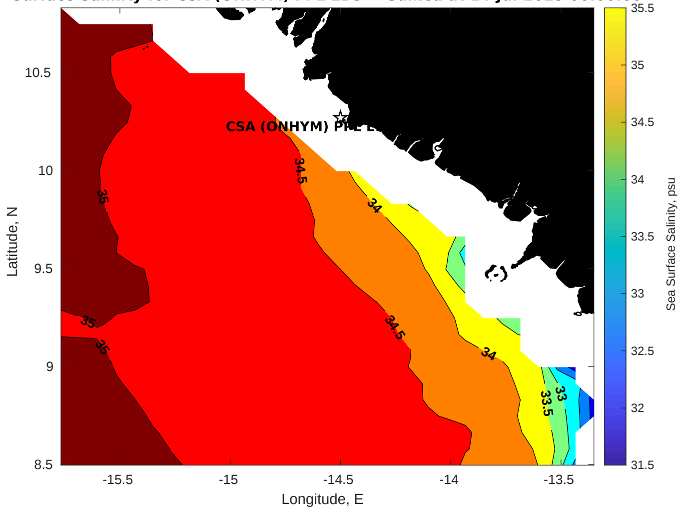
Surface Salinity for CSA (ONHYM) PPL EBS - Guinea at 14-Jul-2025 00:00:00
