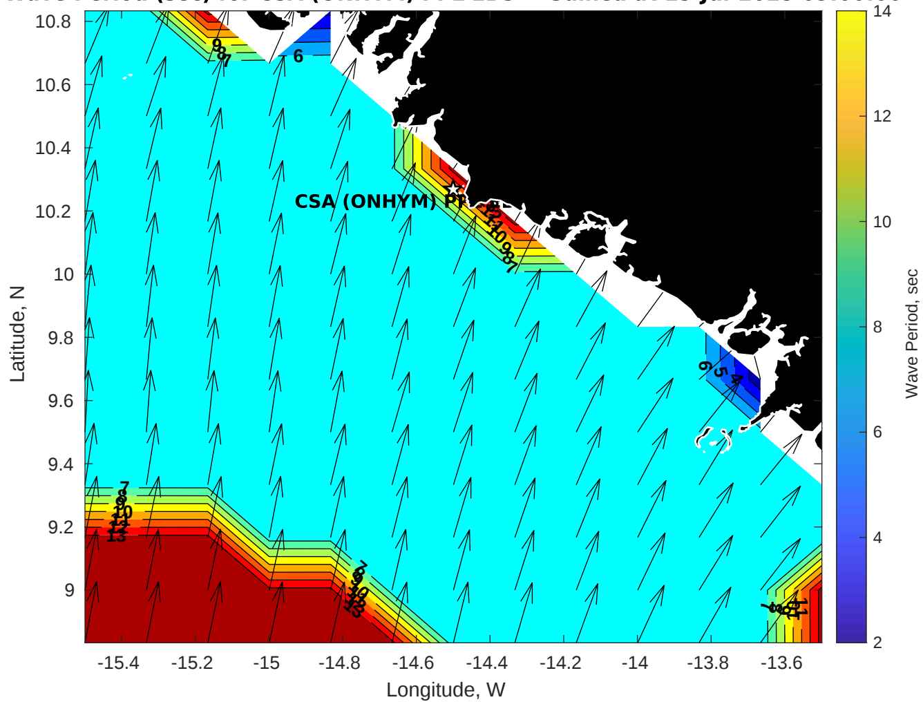
Wave Period (sec) for CSA (ONHYM) PPL EBS - Guinea at 15-Jul-2025 09:00:00
