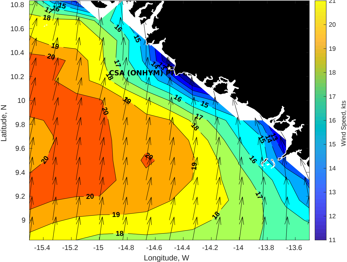
Winds (kts) for CSA (ONHYM) PPL EBS - Guinea at 15-Jul-2025 09:00:00
