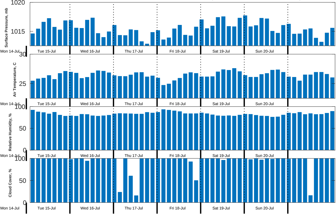
Met Forecast for CSA (ONHYM) PPL EBS - Guinea from 15-Jul-2025 00:00:00 to 22-Jul-2025 00:00:00
