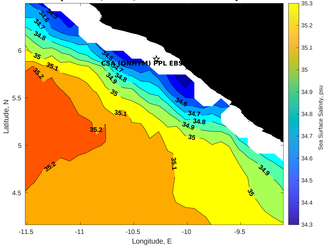
Surface Salinity for CSA (ONHYM) PPL EBS - Liberia at 14-Jul-2025 00:00:00
