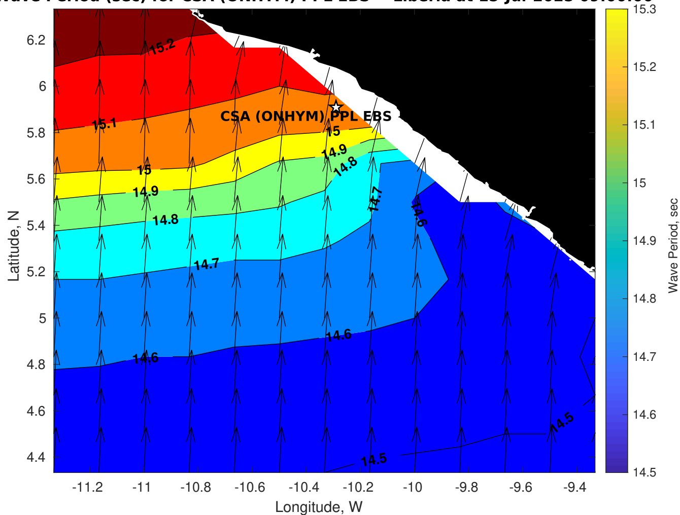
Wave Period (sec) for CSA (ONHYM) PPL EBS - Liberia at 15-Jul-2025 09:00:00
