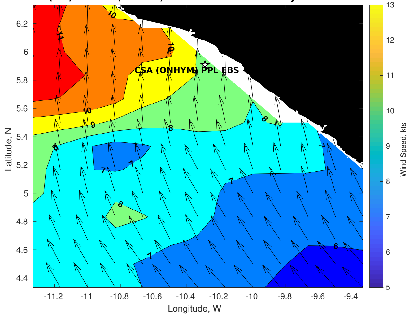
Winds (kts) for CSA (ONHYM) PPL EBS - Liberia at 15-Jul-2025 09:00:00
