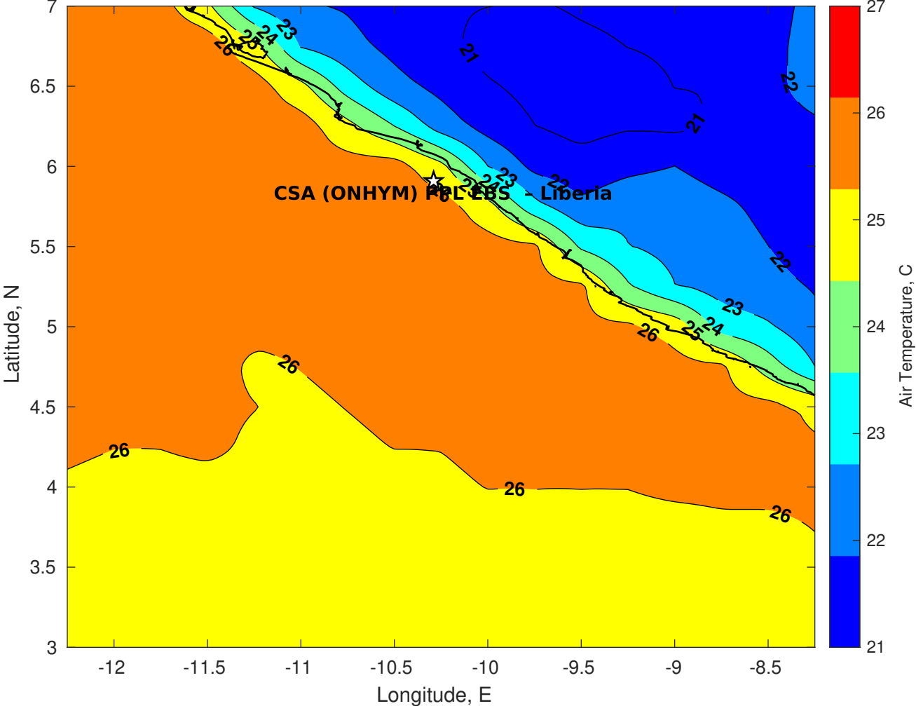
Air Temperature (C) for CSA (ONHYM) PPL EBS - Liberia at 15-Jul-2025
