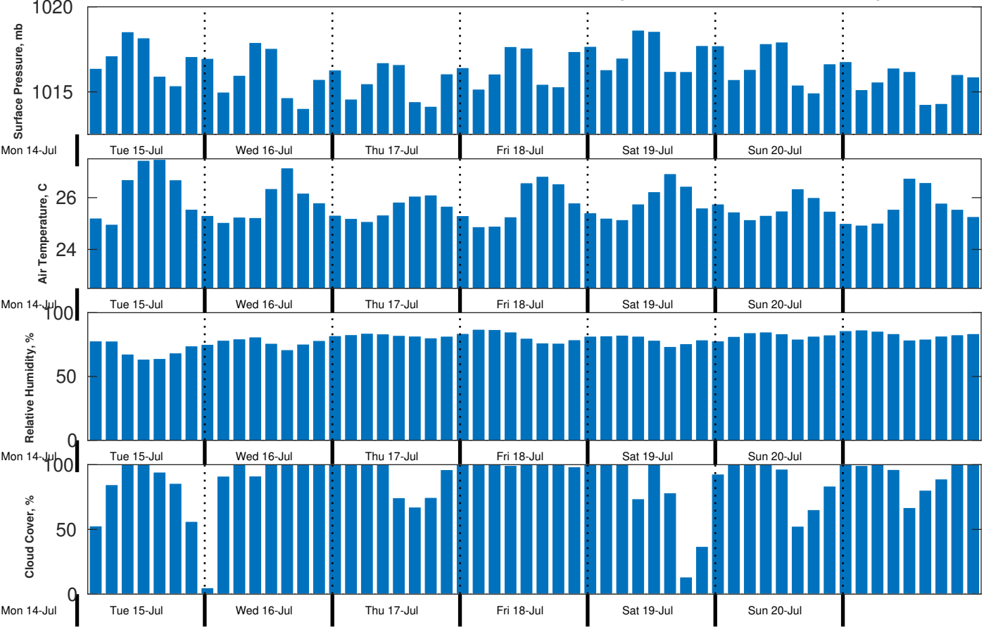
Met Forecast for CSA (ONHYM) PPL EBS - Liberia from 15-Jul-2025 00:00:00 to 22-Jul-2025 00:00:00
