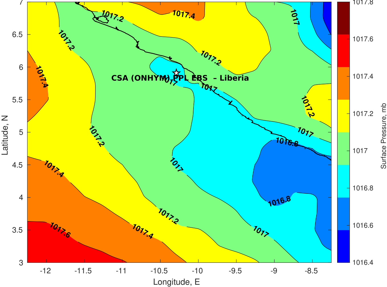
Surface Pressure (mb) for CSA (ONHYM) PPL EBS - Liberia at 16-Jul-2025 00:00:00
