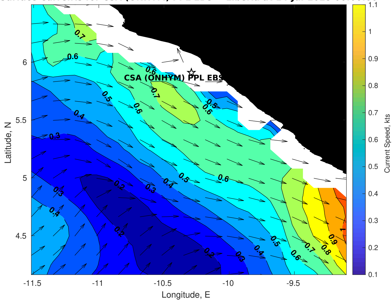
Surface Currents for CSA (ONHYM) PPL EBS - Liberia at 14-Jul-2025 00:00:00
