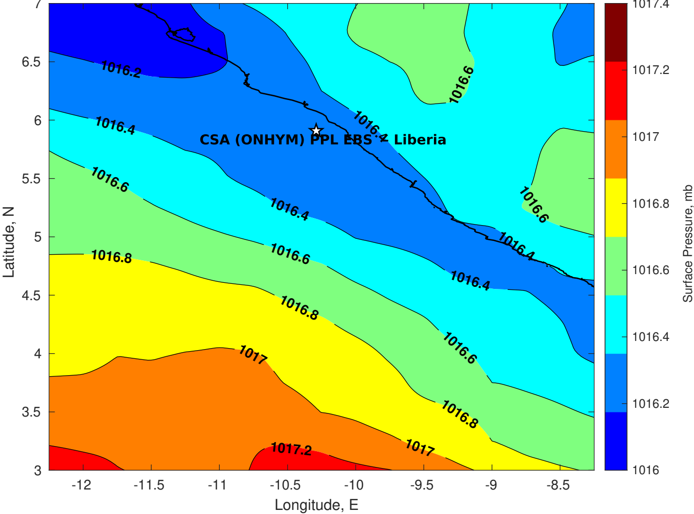
Surface Pressure (mb) for CSA (ONHYM) PPL EBS - Liberia at 17-Jul-2025 00:00:00
