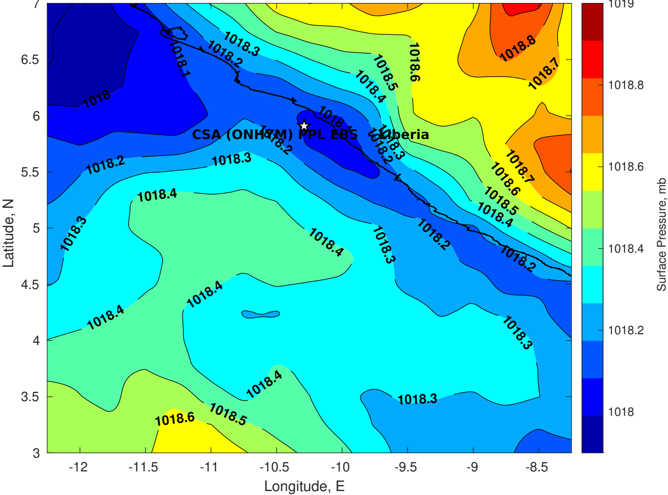
Surface Pressure (mb) for CSA (ONHYM) PPL EBS - Liberia at 15-Jul-2025 00:00:00
