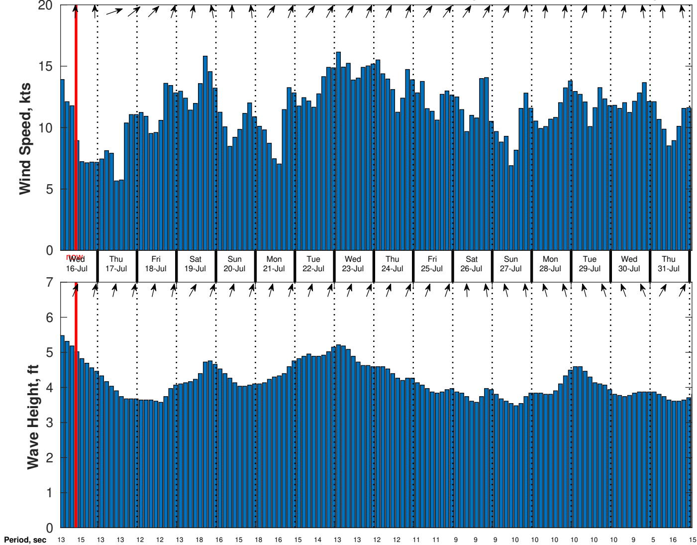
Wind & Wave Forecast for CSA (ONHYM) PPL EBS - Liberia from 15-Jul-2025 01:00:00 to 31-Jul-2025 01:00:00
