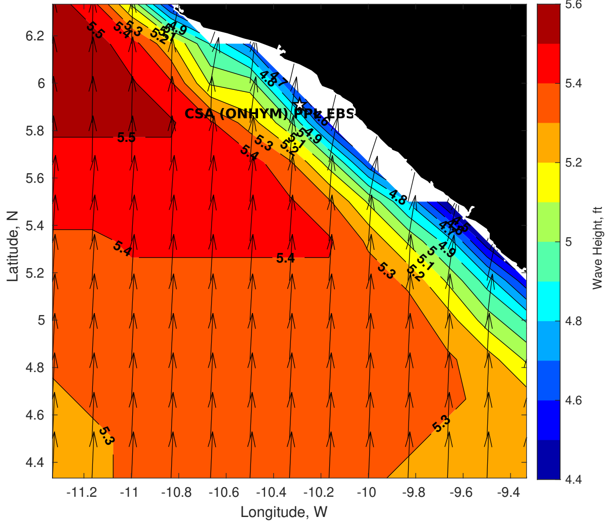
Wave Height (ft) for CSA (ONHYM) PPL EBS - Liberia at 15-Jul-2025 09:00:00
