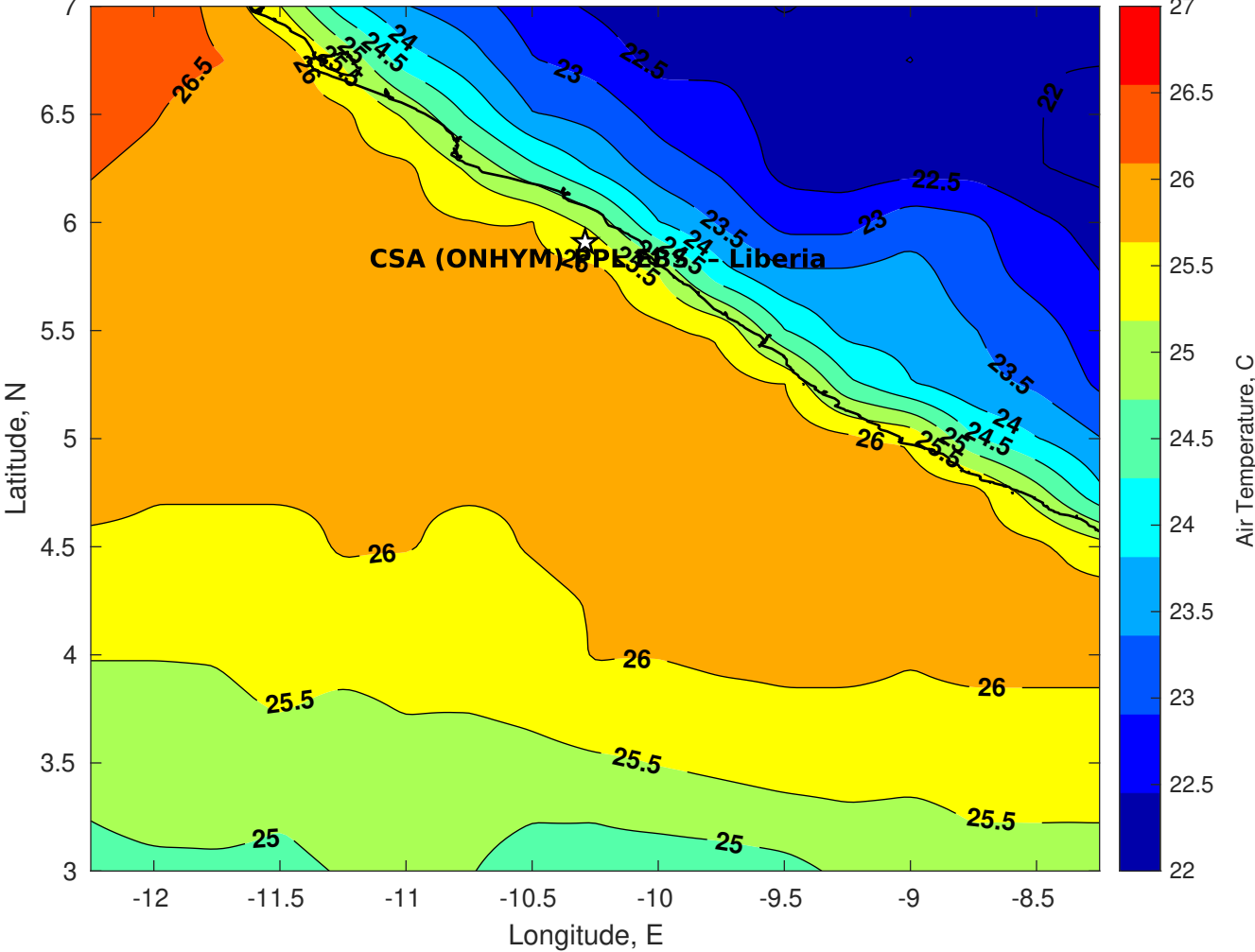
Air Temperature (C) for CSA (ONHYM) PPL EBS - Liberia at 15-Jul-2025
