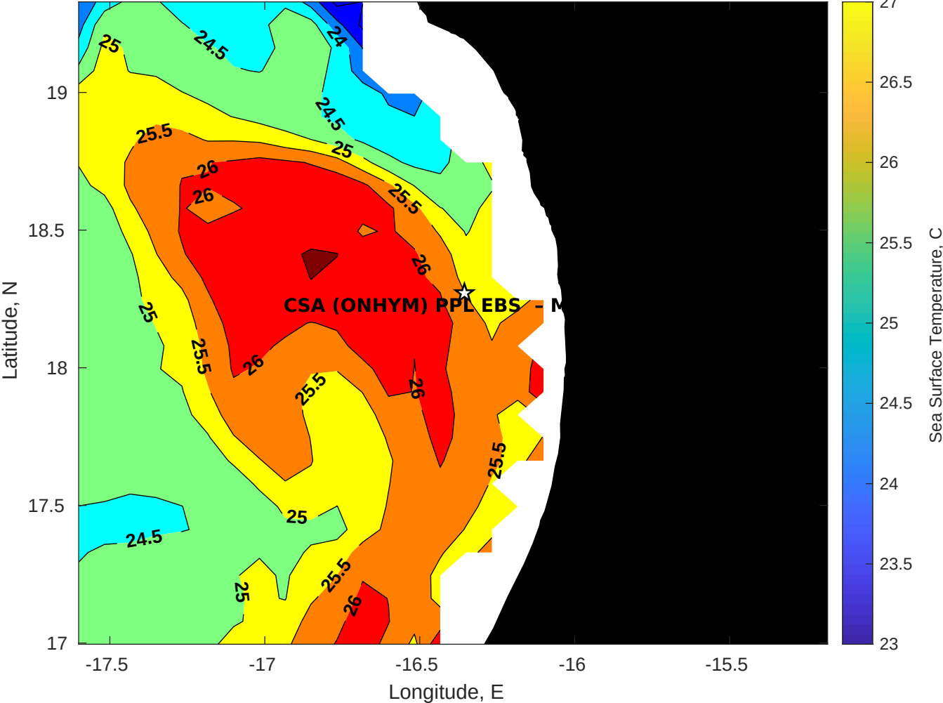
SST for CSA (ONHYM) PPL EBS - Mauritania at 14-Jul-2025 00:00:00
