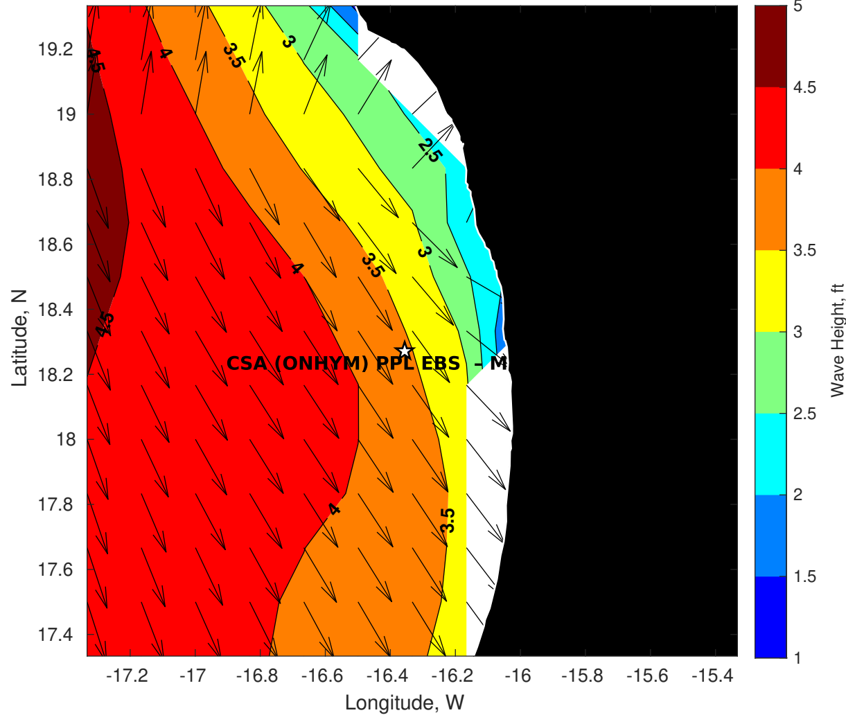
Wave Height (ft) for CSA (ONHYM) PPL EBS - Mauritania at 15-Jul-2025 09:00:00
