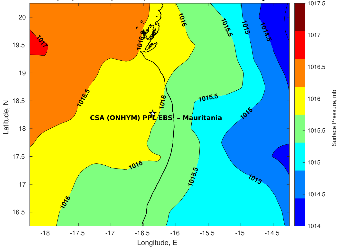
Surface Pressure (mb) for CSA (ONHYM) PPL EBS - Mauritania at 17-Jul-2025 00:00:00
