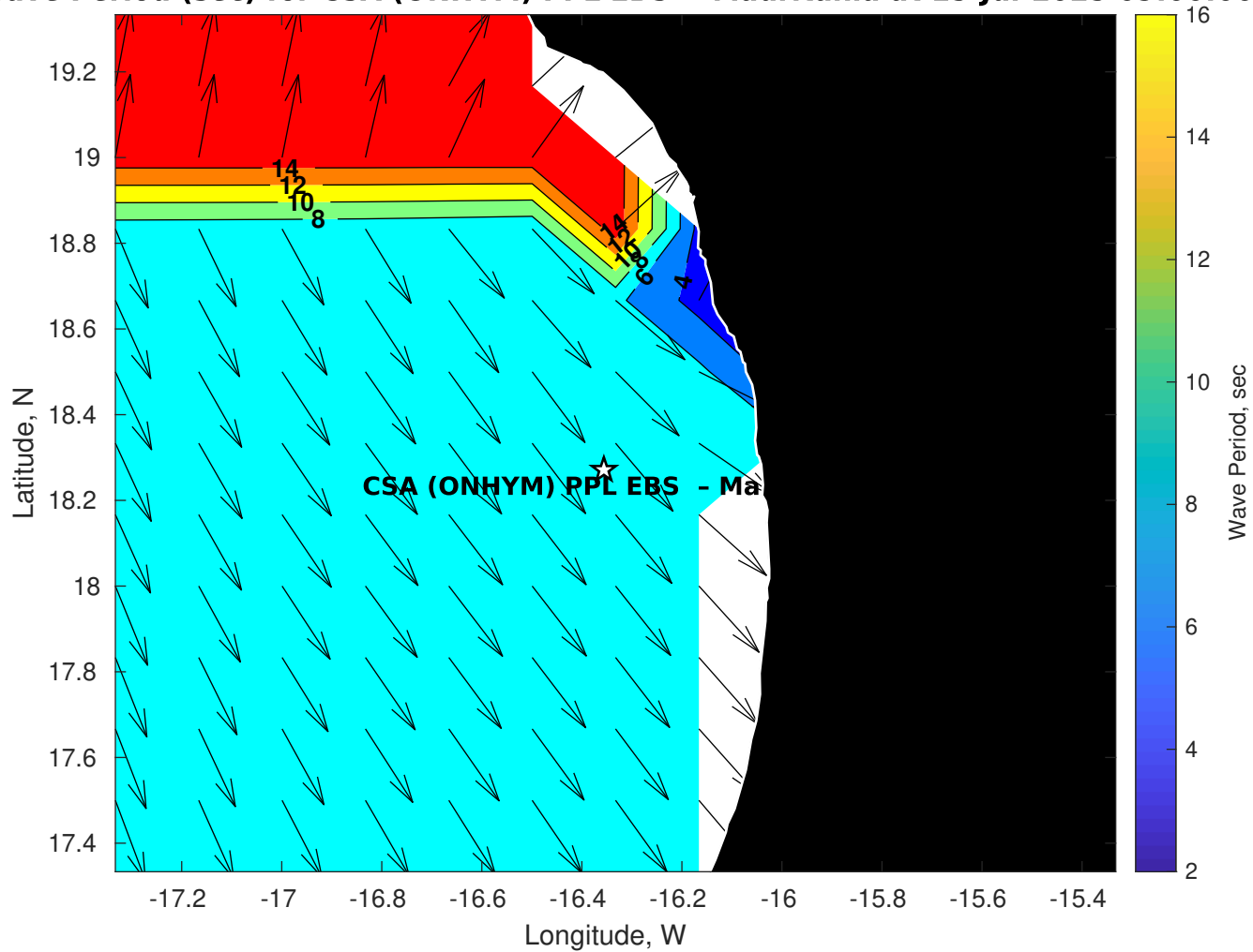
Wave Period (sec) for CSA (ONHYM) PPL EBS - Mauritania at 15-Jul-2025 09:00:00
