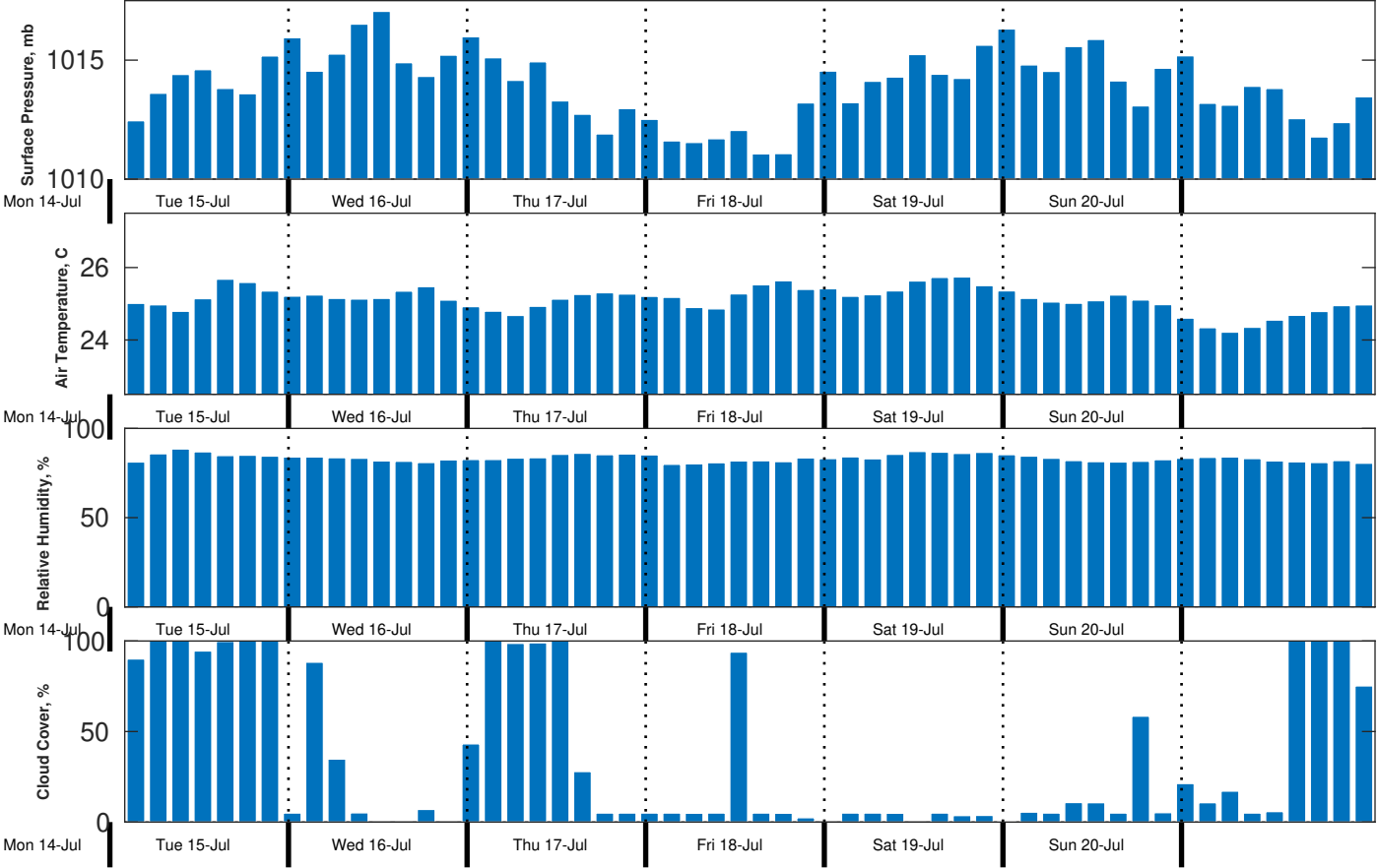
Met Forecast for CSA (ONHYM) PPL EBS - Mauritania from 15-Jul-2025 00:00:00 to 22-Jul-2025 00:00:00
