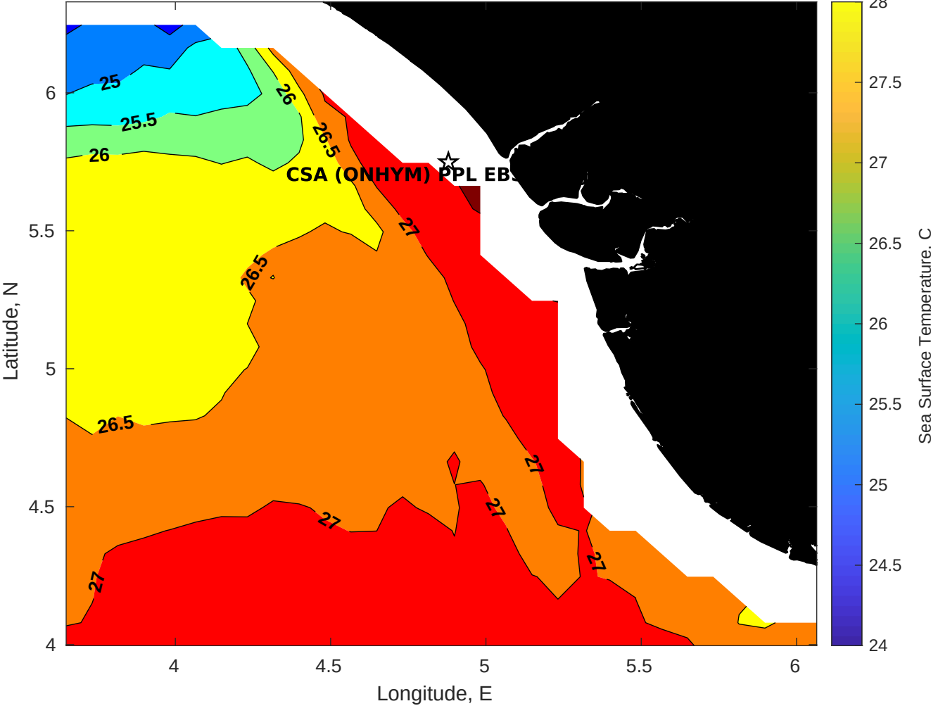
SST for CSA (ONHYM) PPL EBS - Nigeria at 14-Jul-2025 00:00:00
