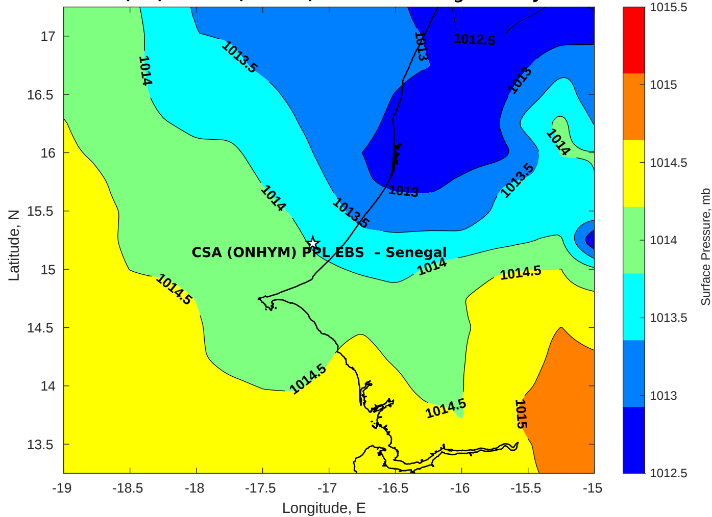
Surface Pressure (mb) for CSA (ONHYM) PPL EBS - Senegal at 15-Jul-2025 00:00:00
