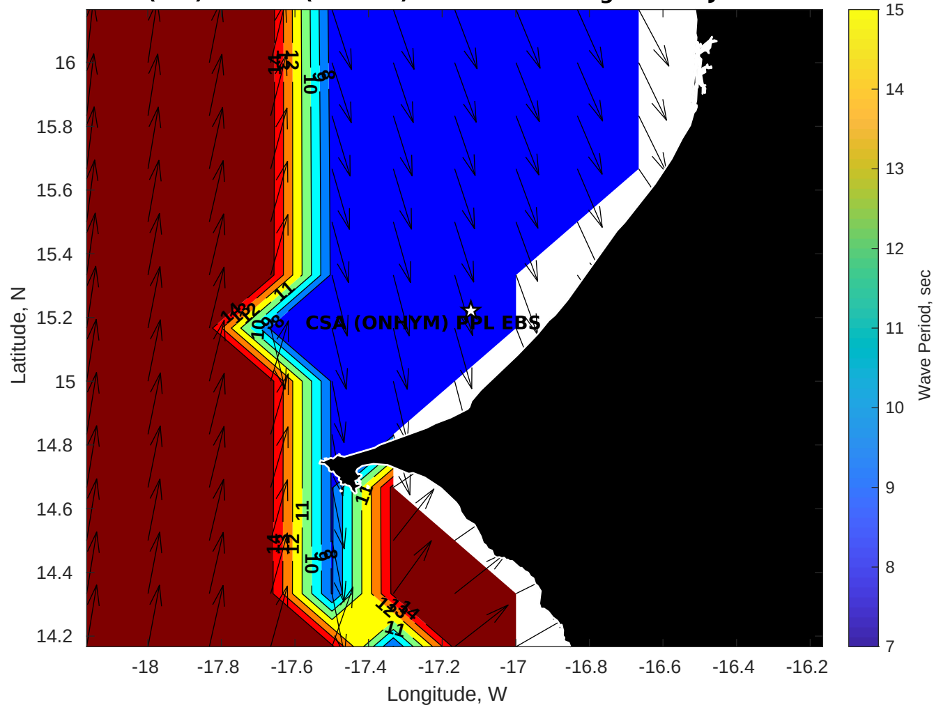
Wave Period (sec) for CSA (ONHYM) PPL EBS - Senegal at 15-Jul-2025 09:00:00
