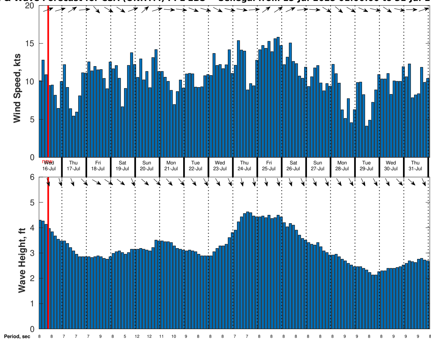
Wind & Wave Forecast for CSA (ONHYM) PPL EBS - Senegal from 15-Jul-2025 01:00:00 to 31-Jul-2025 01:00:00
