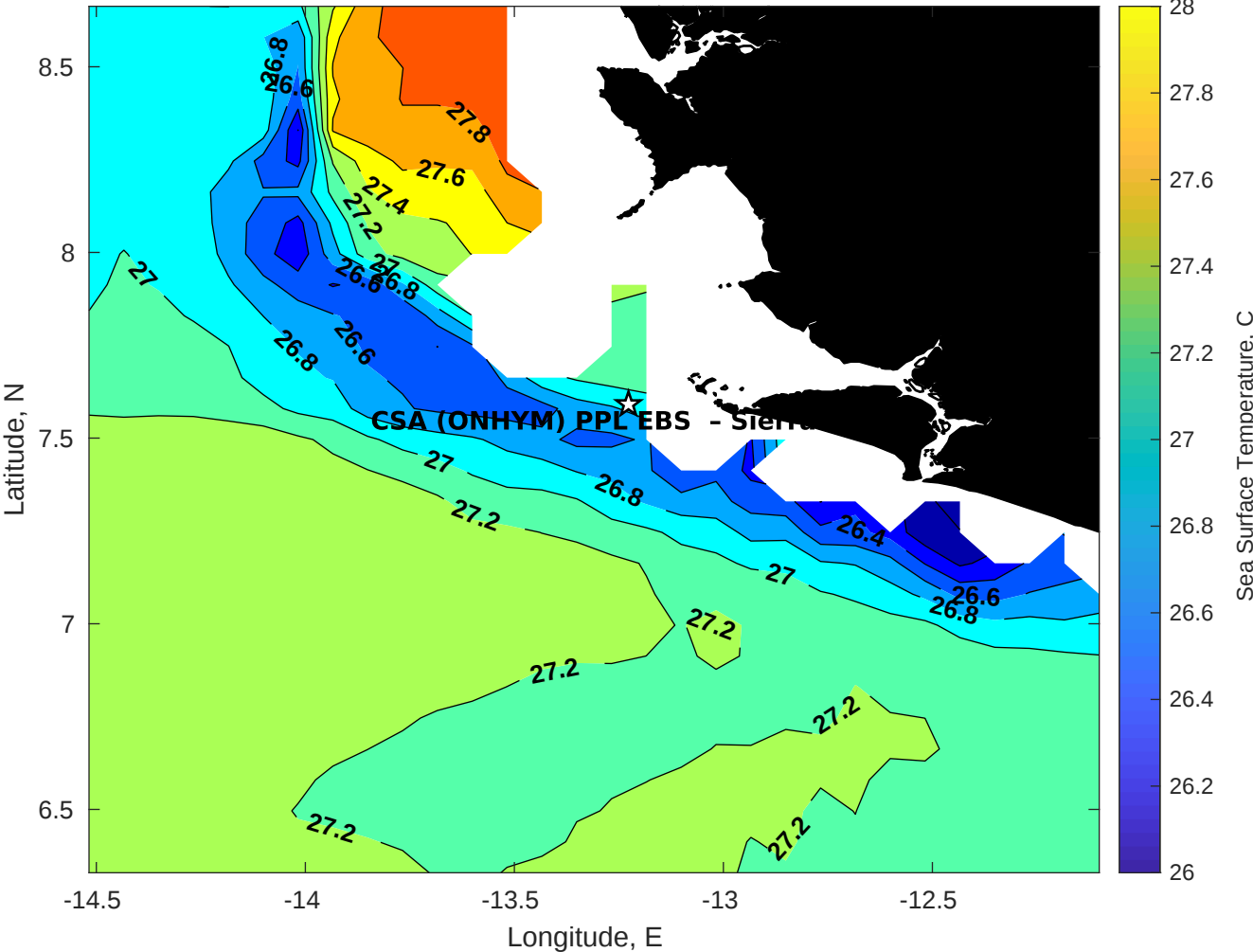
SST for CSA (ONHYM) PPL EBS - Sierra Leone at 14-Jul-2025 00:00:00
