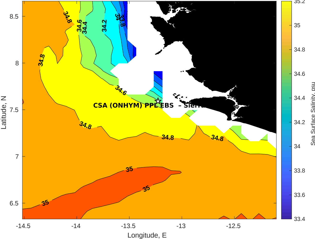
Surface Salinity for CSA (ONHYM) PPL EBS - Sierra Leone at 14-Jul-2025 00:00:00
