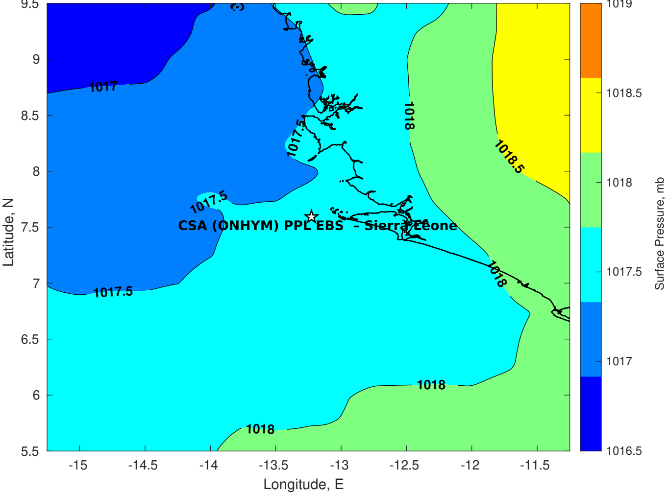
Surface Pressure (mb) for CSA (ONHYM) PPL EBS - Sierra Leone at 15-Jul-2025 00:00:00
