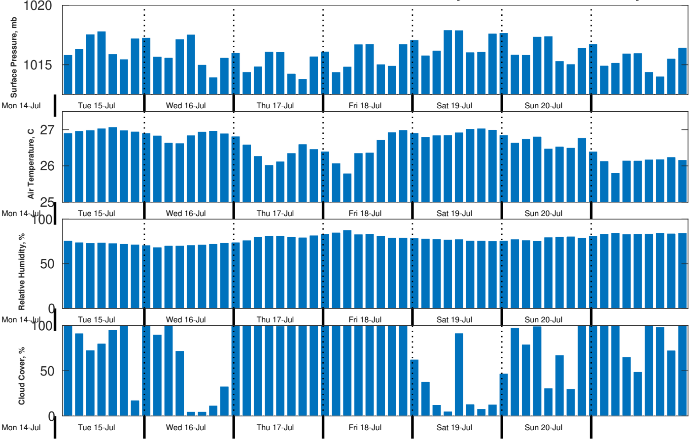
Met Forecast for CSA (ONHYM) PPL EBS - Sierra Leone from 15-Jul-2025 00:00:00 to 22-Jul-2025 00:00:00
