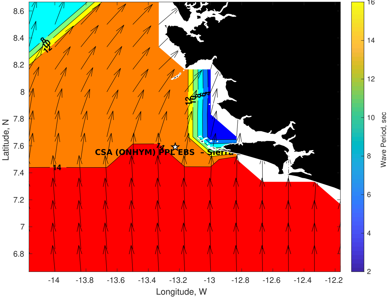
Wave Period (sec) for CSA (ONHYM) PPL EBS - Sierra Leone at 15-Jul-2025 09:00:00
