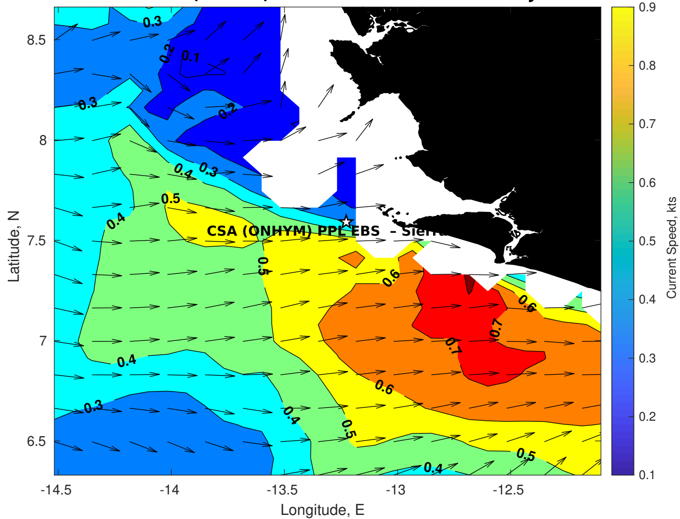
Surface Currents for CSA (ONHYM) PPL EBS - Sierra Leone at 14-Jul-2025 00:00:00
